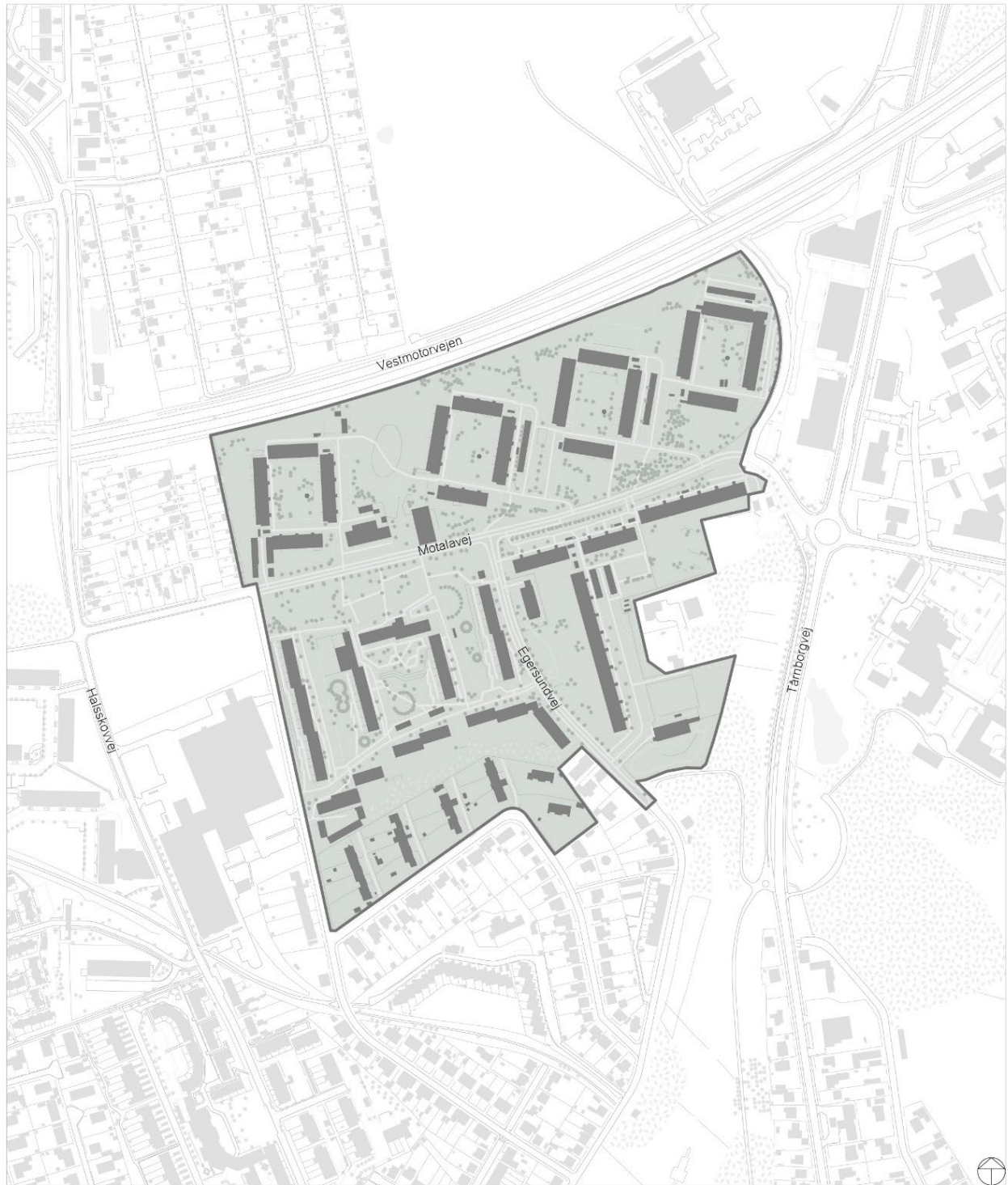
Figur 2. Motalavej, situationsplan 1:5000.
