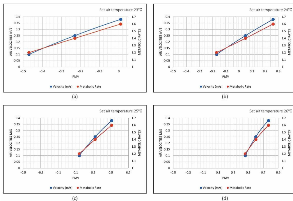
Figure 15. Impact of temperature on thermal comfort for occupants with different metabolic rates. (a–d): different occupants.
