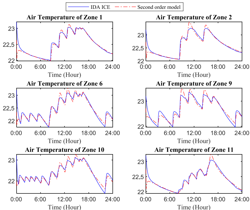
Fig. 4. 1-step ahead prediction by the second order model ( T_s = 5 min).
