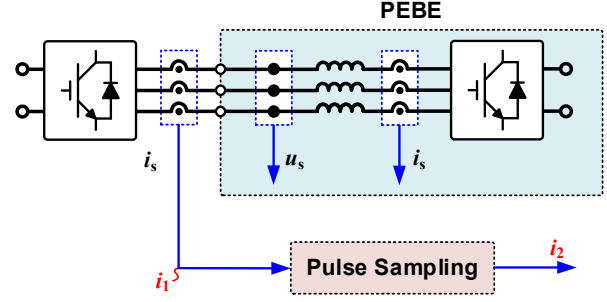
Fig. 17. Analog-to-Digital Conversion
