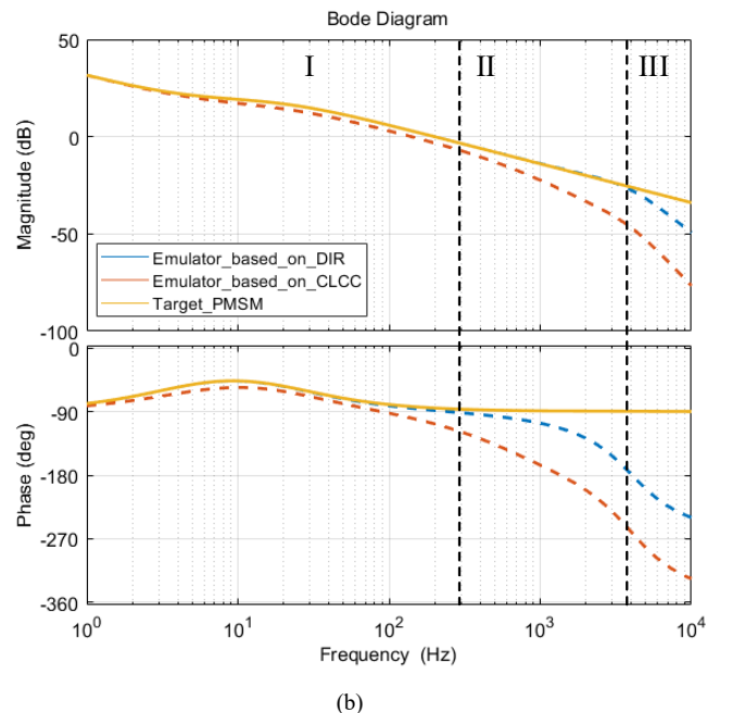
Fig. 9. Electric machine emulation based on Direct Impedance Regulation. (a) Circuit configuration. (b) Bode diagram.
