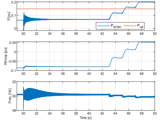
Fig. 10. WT group WTB: Active power reference, P_{ref} , and generated active power, P_{WTB1} , (top), droop power reference and PLL frequency during OHL energization and connection of block load.
