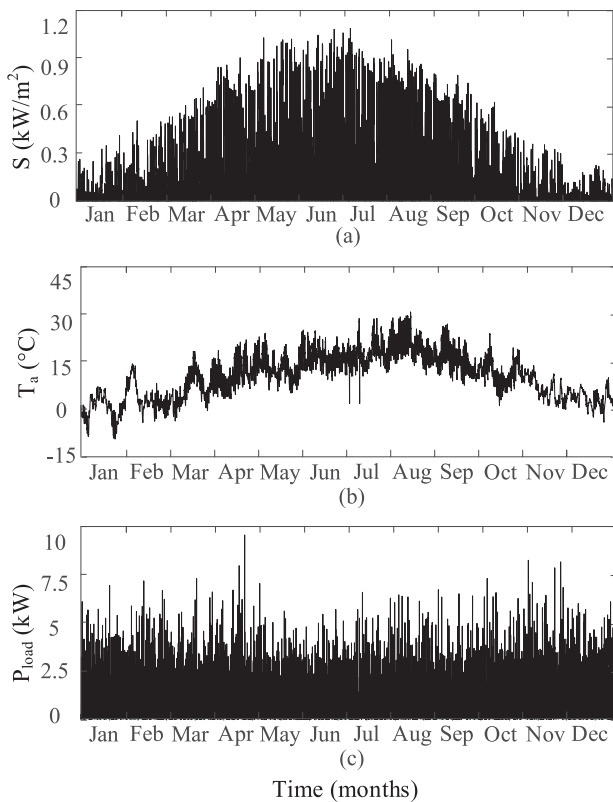
FIG. 7. A one-year mission profile of the PV-battery system installation site in Germany: (a) solar irradiance S , (b) ambient temperature T_a , and (c) load demand P_{\text{load}} .
