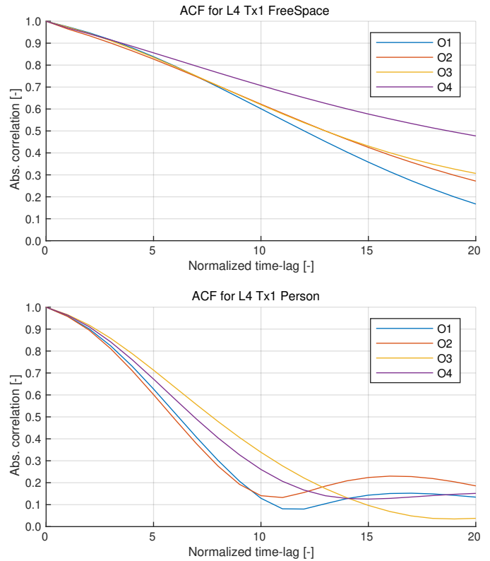
Fig. 1. Estimated ACF curves for different orientation in the scenario L4, Tx1, (top) in free space and (bottom) with person. The time-lag is normalized to the 5 ms sampling interval.
