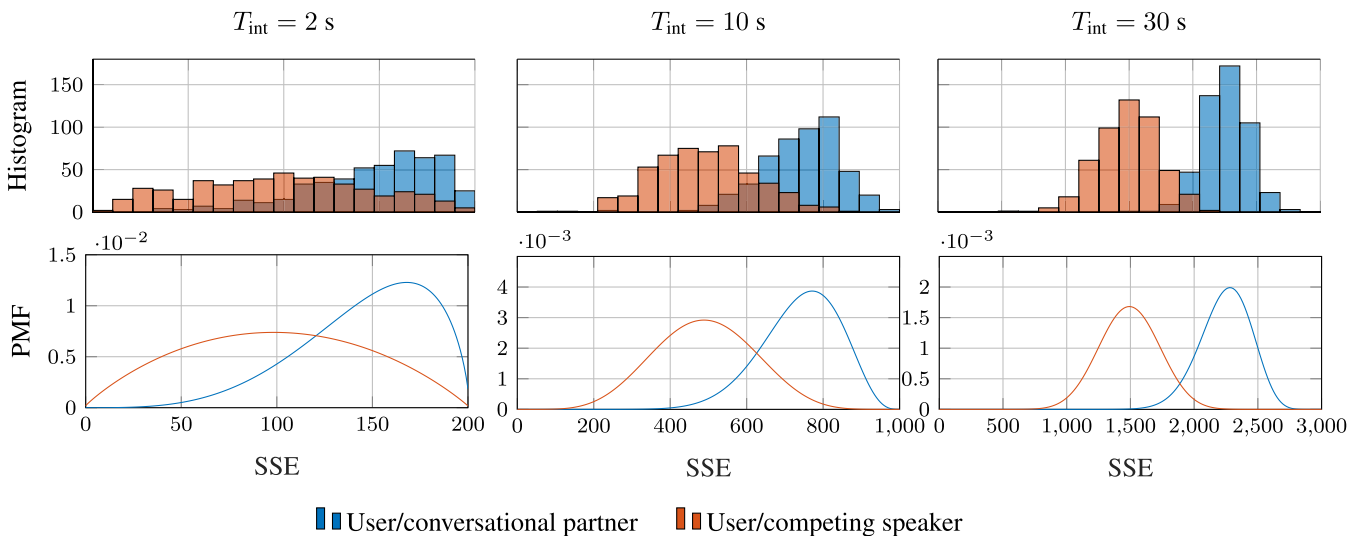
FIGURE 3. Histograms of K = 500 observations of SSEs from real conversations are shown in the upper plots. The bottom plots show beta-binomial distributions where the parameters are found from the observations. In all plots the blue color denotes the conversational partner and the red color denotes the competing speaker.
