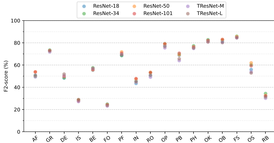
(a) Per-class performance for all MSHViT models.
