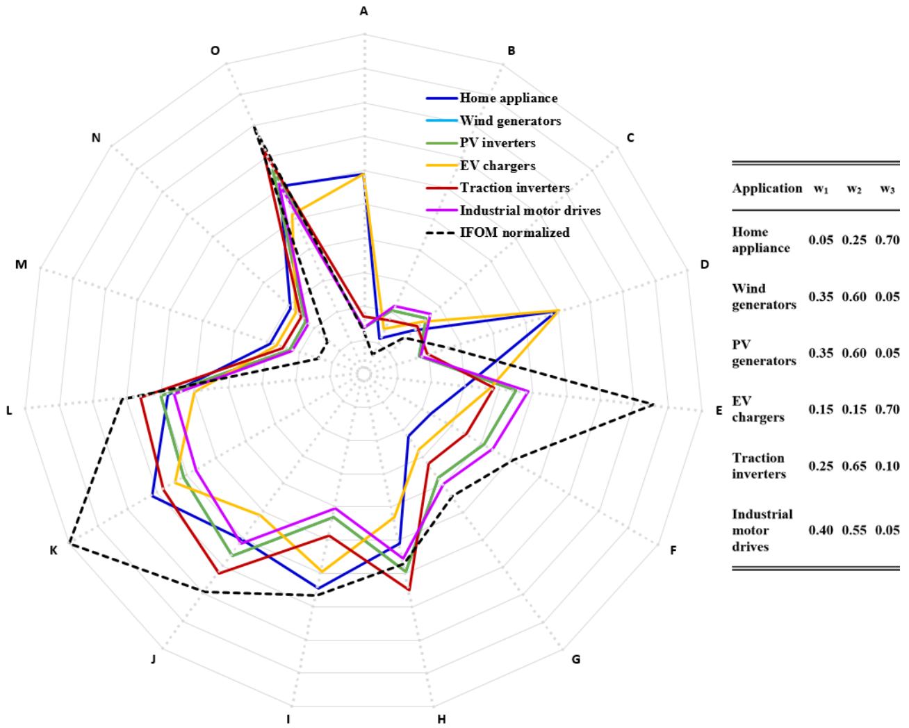
Figure 4. Normalized IFOM and application-based FOM (in different applications) assigned to the CMMs
