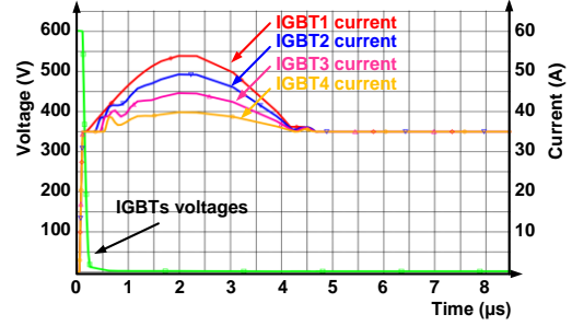
Fig. 7. IGBTs currents and voltages when the IGBTs are in the turn-on state.
