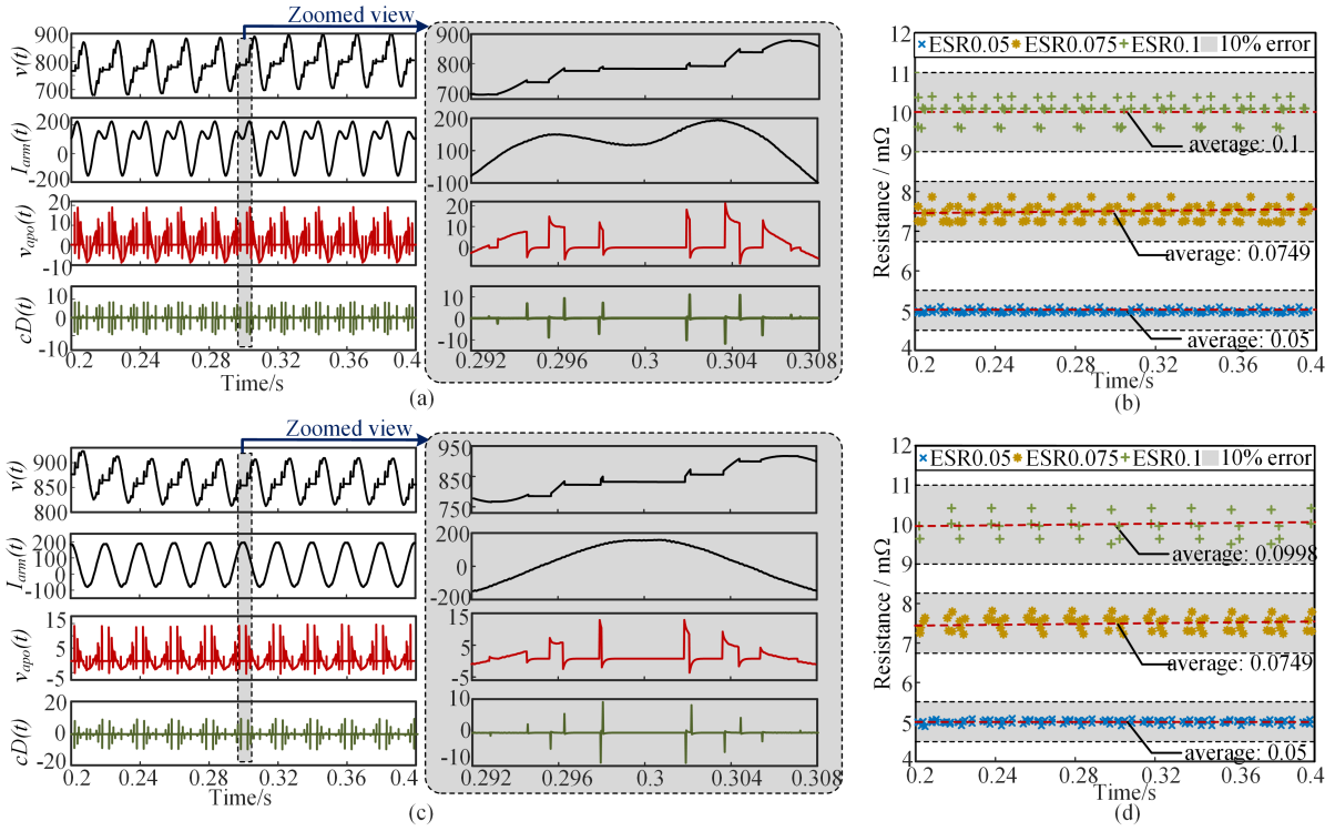
Fig. 8. Extracted signals and ESR estimation results with PSC modulation in the simulation. (a) without circulating current suppressing control and (b) the corresponding estimated ESR. (c) with circulating current suppressing control and (d) the corresponding estimated.
