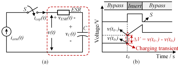
Fig. 3. Capacitor charging transient analysis. (a) simplified circuit. (b) capacitor terminal voltage during the charging transient.
