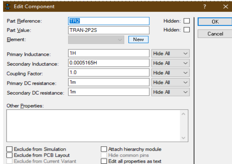
Figure 2. Transformer designing
