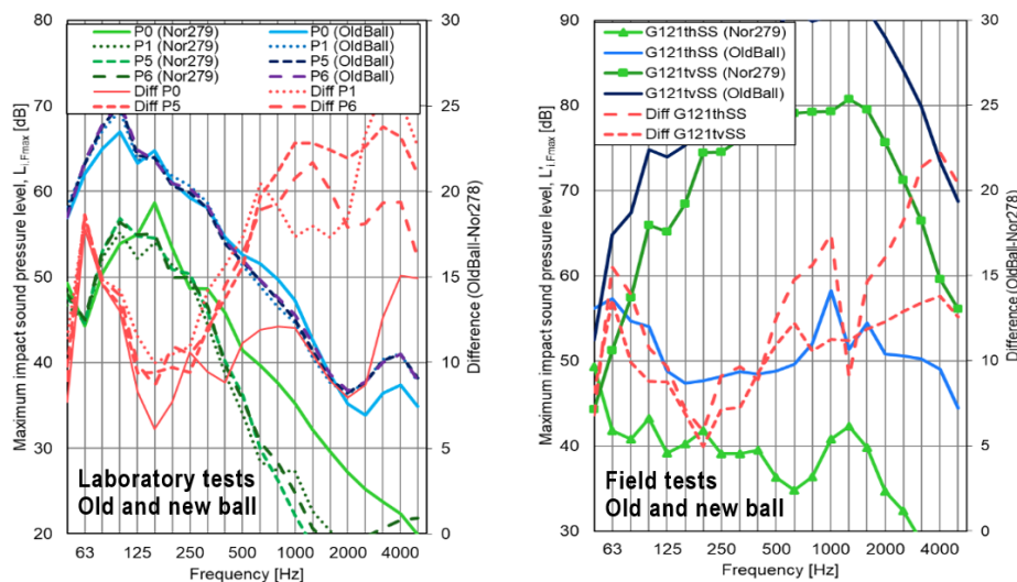
Figure 7 – Comparison of the two impact balls in laboratory L_{i,Fmax} (left) and field L'_{i,Fmax} (right). The red curves show the differences between the old and new ball.
