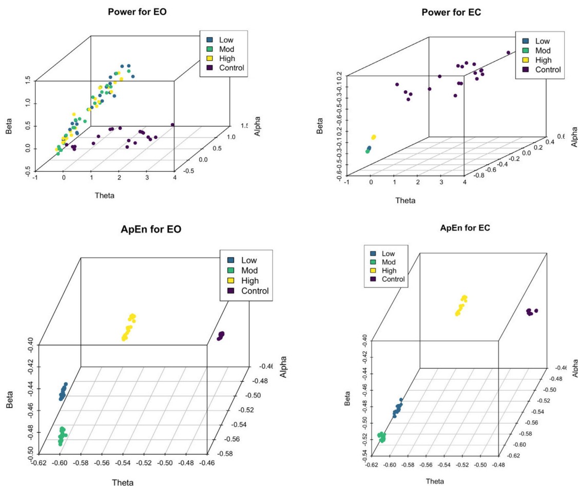
Fig. 8. 3D Spatial distribution of ApEn and power in theta, alpha, and beta band. ApEn clusters the 22 electrodes of NP severities and control group, whereas power does not. Data was normalized in a z-score scale with a center of 0 and a standard deviation of 1. Mod represents moderate severity.
