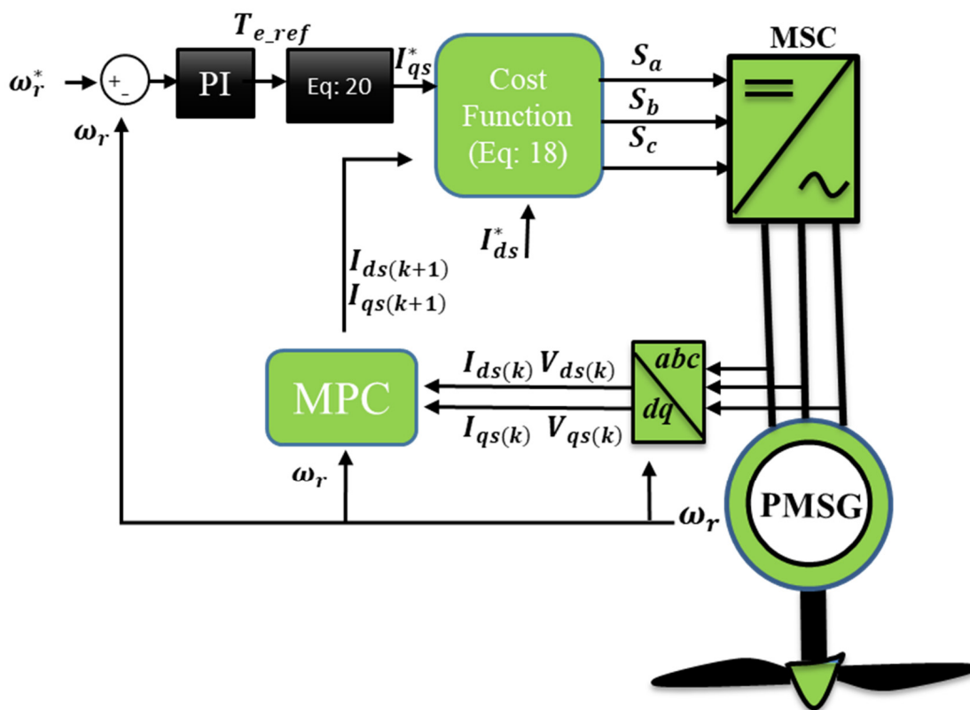
Figure 4. MSC with proposed FCS-MPC scheme.
