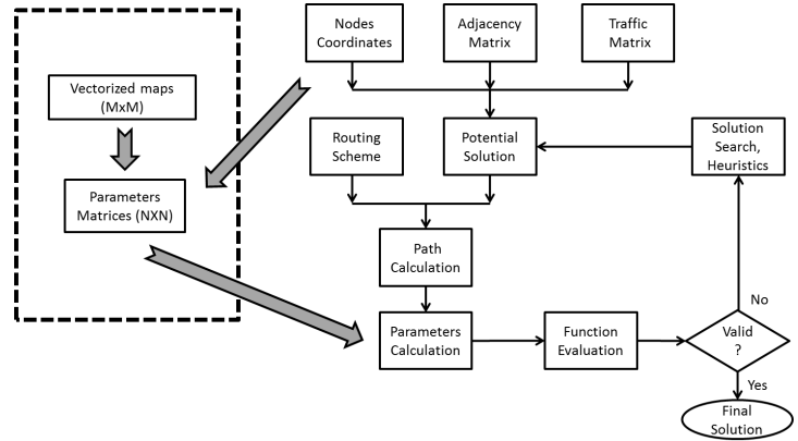
Fig. 1. System Scheme
