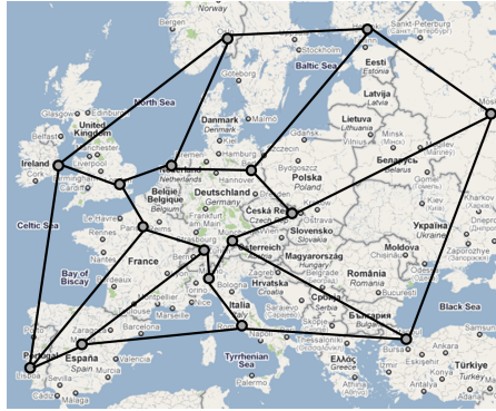
Fig. 5. Constant Factor Solution, FL_{ij} = \sqrt{2} , NT 1
