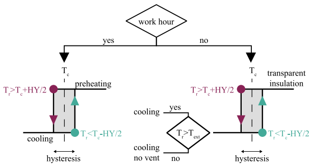
Fig. A.12. Outline of airflow-pattern control for I-DIFFER: HY = hysteresis (summer: 4 °C; winter: 2.5 °C); T_{ext} = ambient air temperature; T_c = thermal neutral temperature dependent on season (summer: T_c = T_c - 0.5 °C; winter: T_c = T_c ), T_{op} = classroom operative temperature. Based on Bugenings et al. [24].
