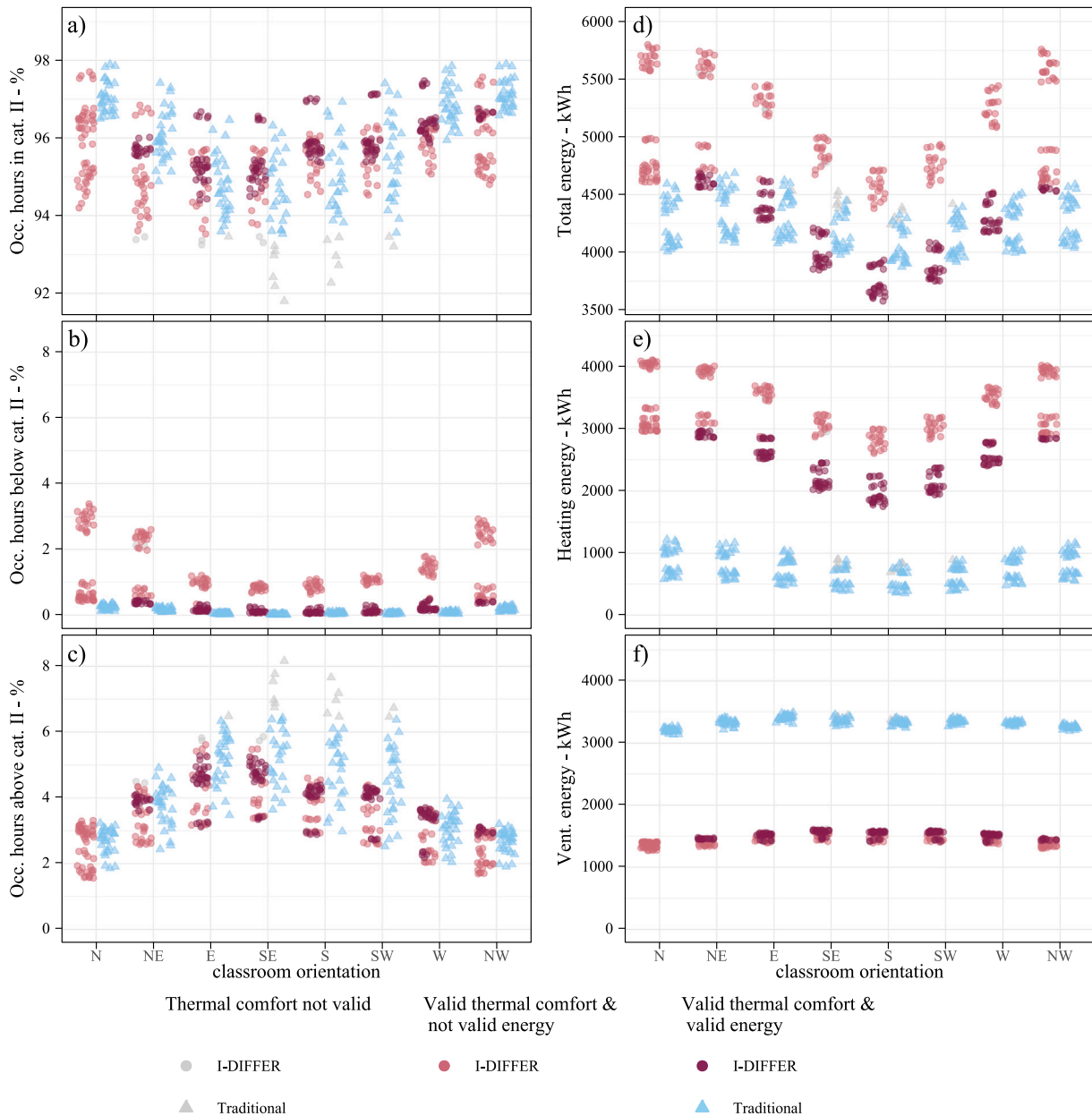
Fig. 4. Orientation: Occupied hours inside cat. II, occupied hours below cat. II, occupied hours above cat. II, total PE, PE heating and PE ventilation. Traditional n = 30; I-DIFFER n = 50 (per orientation).
