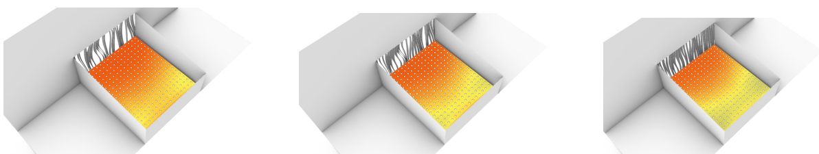
Figure 8. Daylight autonomy simulation. (Left) High open ration of the facade with Mean daylight factor - 2.1% (Center) Medium open ratio with Mean daylight factor - 1.9% (Right) Low open ration with Mean daylight factor - 1.6%
