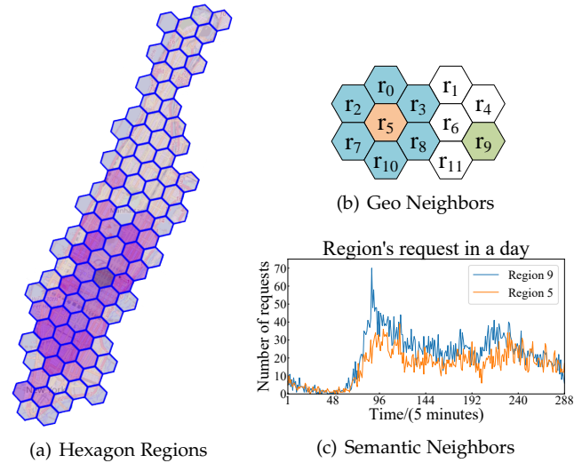
Fig. 2. (a) The hexagon regions of Manhattan. Dark colors indicate high demands. (b) The geographical neighbors of r_5 are r_0, r_2, r_3, r_7, r_8, and r_{10} . (c) Since r_9 and r_5 have similar request patterns, they are semantic neighbors.
