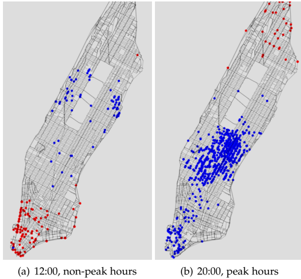
Fig. 5. The real-time locations of requests and idle agents in peak and non-peak hours (red dot: idle agent, blue dot: request).
