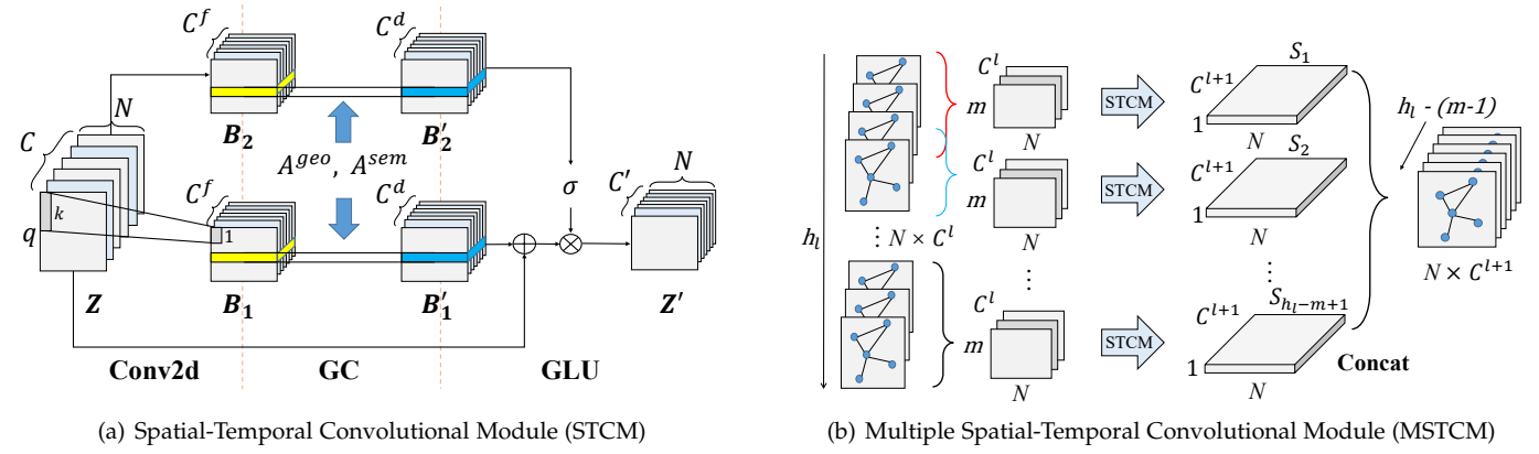
Fig. 4. Spatial-Temporal Gated Block
