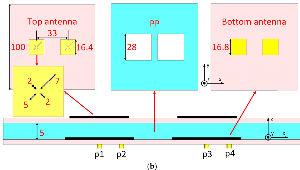
Figure 4. (a) Design procedure of the isolation improvement for dual-element dual-polarized antenna array with NRMS. Array 1 is the reference antenna array. In the next step, Array 2 is depicted, where a metasurface consisting of periodic cross metal rings with a period T is employed above Array 1, where the air cavities with a period 2 \times T are engraved on the metasurface. (b) The configuration of the reference array in the design procedure. (Unit: mm).
