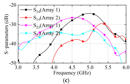
Figure 5. The S parameters of array1 and the one after adding MS and NRMS for array2 and array3, (a) the S_{11} and S_{31} , (b) S_{22} and S_{42} , and (c) S_{14} and S_{23} .
