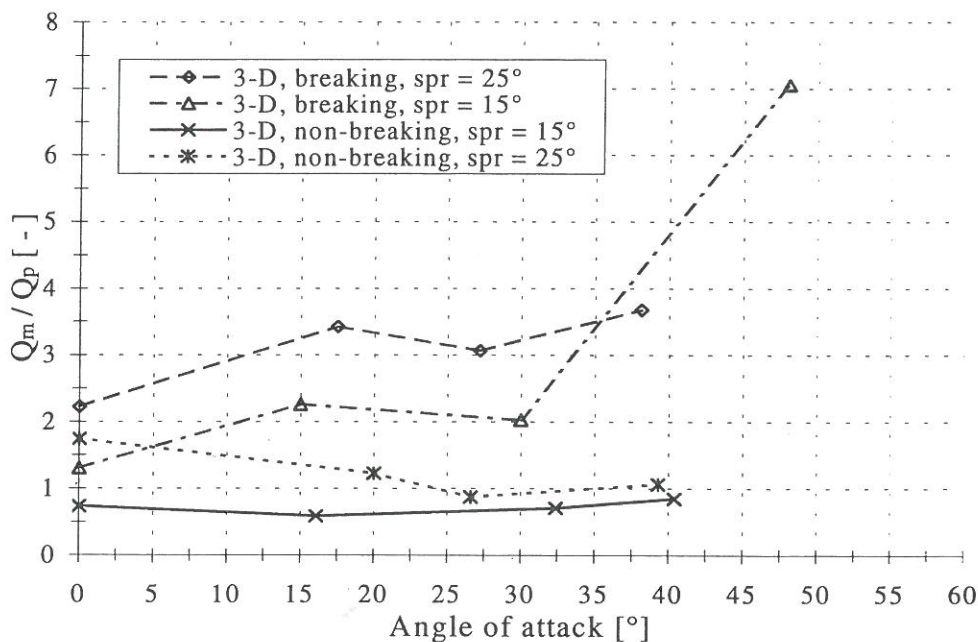
Figure 10 – Comparison of measured and predicted wave overtopping (wave heights at the structure).
