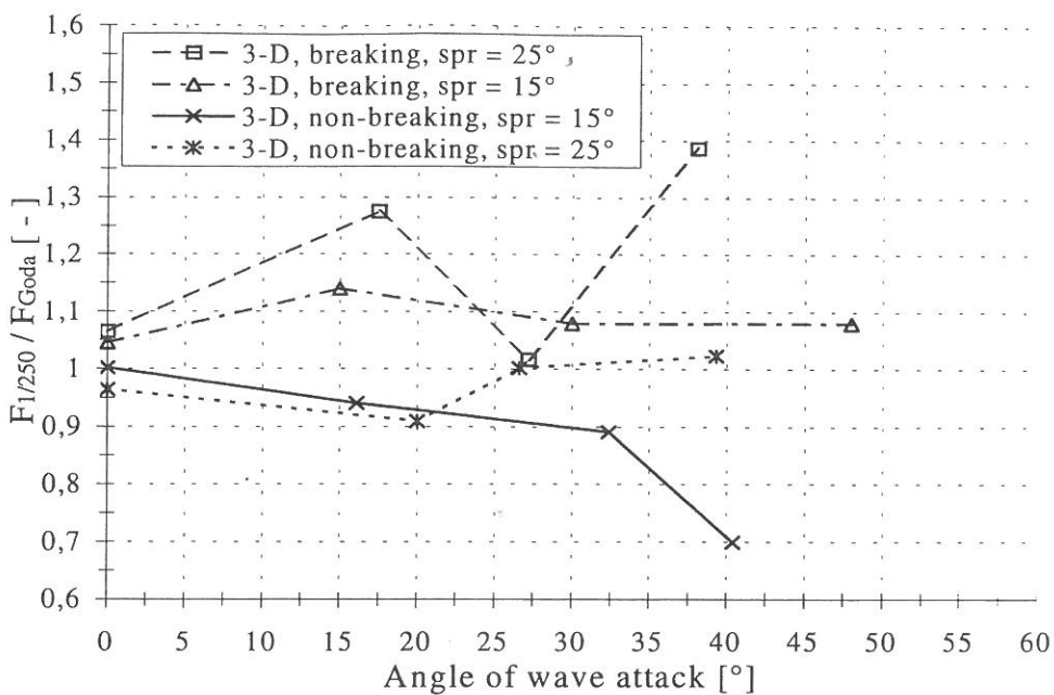
Figure 9 – Comparison with Goda predicted forces (wave heights at the structure).
