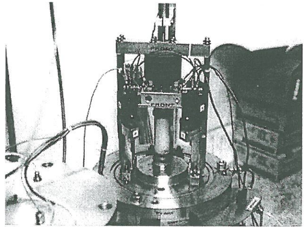
Fig. 4 Detail of the loading system in resonant column device. Supporting frame for the magnets and coils and the top part is shown.
