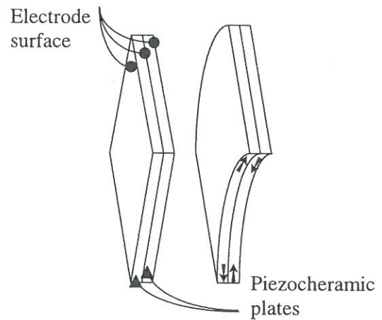
Fig. 6 Principle of single bimorph piezoceramic bender element. Relaxed element at left and excited element at right.
