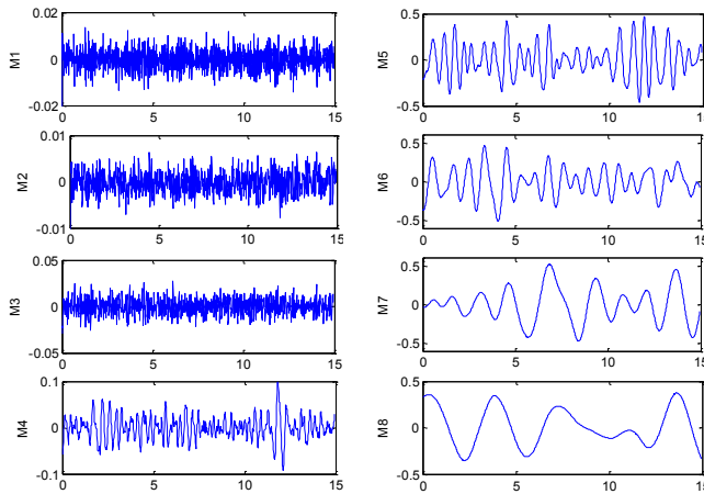
Figure 7-6 Obtained IMFs ( M_i ) after employing CEEMDAN on the vibrating signal ( V ).
