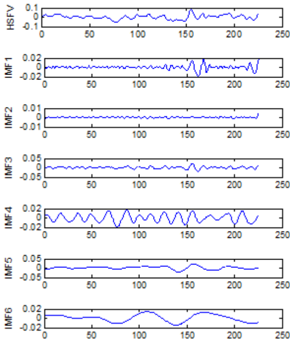
Figure 9-3 An example of first 6 IMFs with obtained for a HSFV of a real face.
