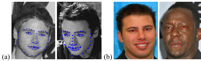
Figure 4-1 Examples of facial landmarks detection: (a) Fast-SIC detected 66 points [2] and (b) SDM detected 49 points in four images of the LFPW database [14].
