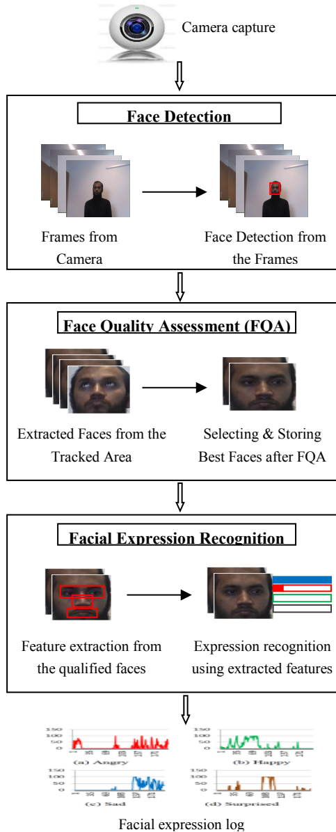
Figure 11-6 The block diagram of the proposed facial expression log construction system with face quality assessment.
