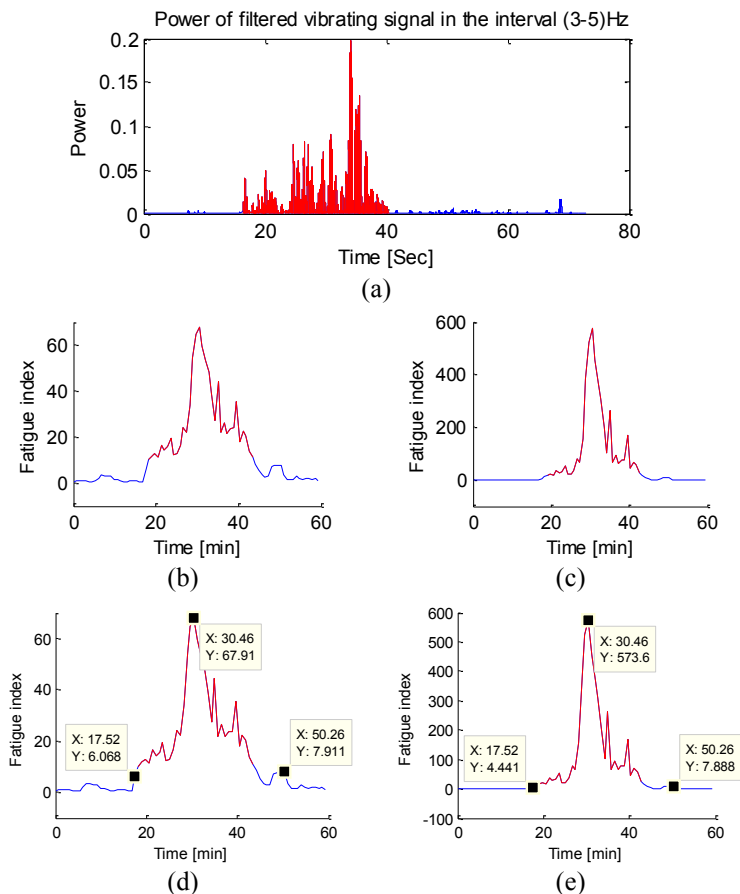
Figure 6-4 Analyzing trajectory for fatigue detection: (a) The power of the trajectory where the blue region is the resting time and the red region shows the fatigue due to exercise in the interval (16.3–40.6) seconds, (b) and (c) before and after using a bipolar sigmoid function to suppress the noise peaks, respectively, and (d) and (e) depicts the effect of bipolar sigmoid in values corresponding to (b) and (c), respectively.
