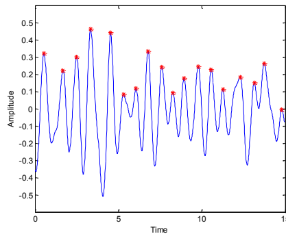
Figure 7-7 Heartbeat peak detection in the 6-th IMF.
