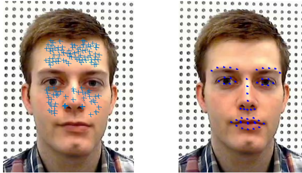
Figure 5-1 Different facial feature tracking methods: (a) facial feature points extracted by the good feature to track method and (b) facial landmarks obtained by the supervised descent method. While GFT extracts a large number of points, SDM merely uses 49 predefined points to track.
