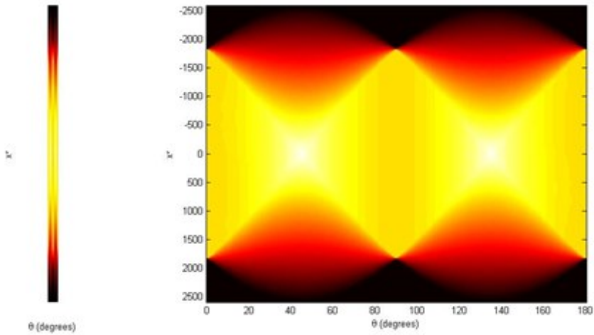
Figure 10-5 The Radon image obtained from the waterfall diagram of Figure 10-4. The discriminative features for the identification purposes are extracted from such Radon images [45]. The image on the right is the zoomed version of the one on the left.
