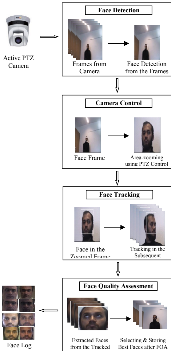
Figure 3-2 Block diagram of the proposed facial image acquisition system with face quality assessment.
