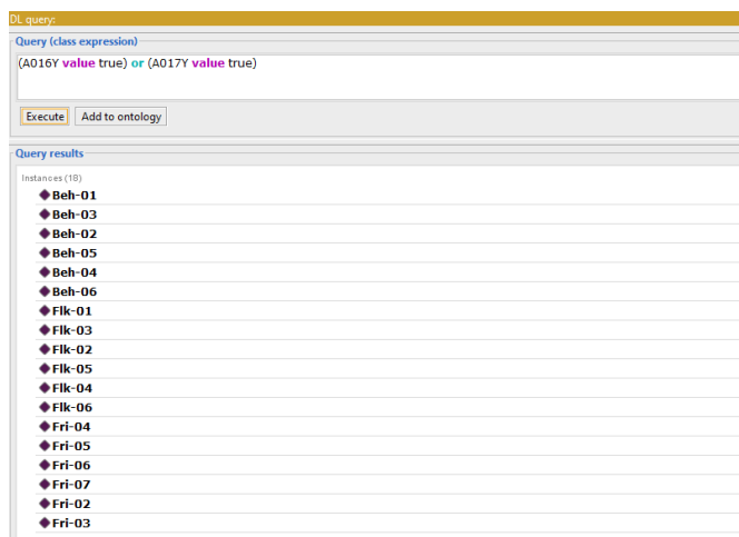
Figure 2. A DL Query as whether there are any individuals that has answered yes to the question 16 or 17. It turns out that 18 of 19 professionals have experienced a calling through a decisive event or through a number of specific events.
