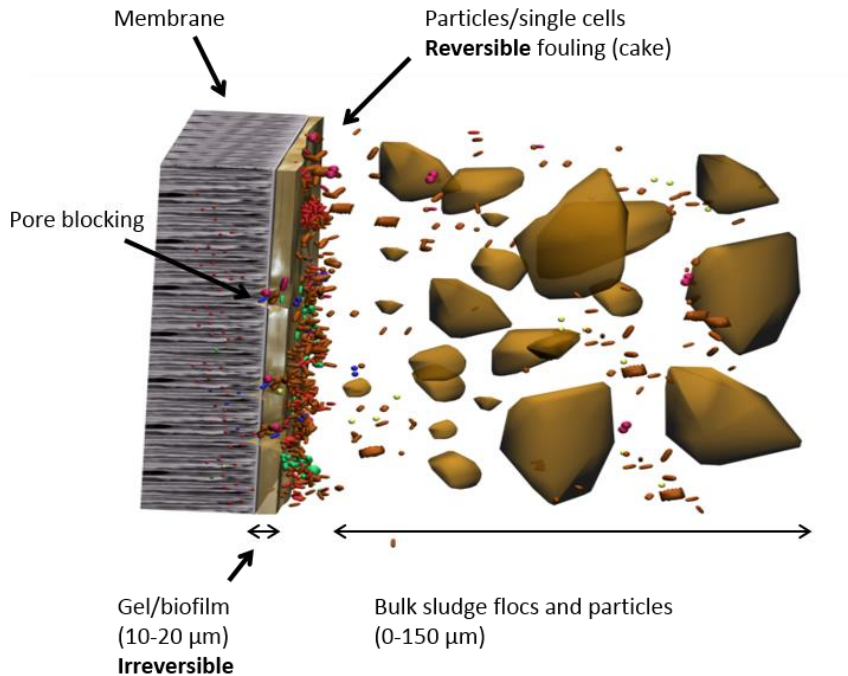
Figure 3 - Fouling model of activated sludge in MBRs, adapted from Hansen et al. (2015).
