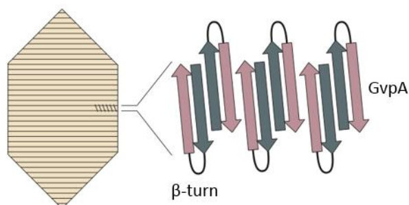
Figure 11 - Assumed aggregation of gas vesicle particle (GvpA) with the characteristic \beta -sheets in the ribs of the gas vesicle. From Pfeifer (2012).
