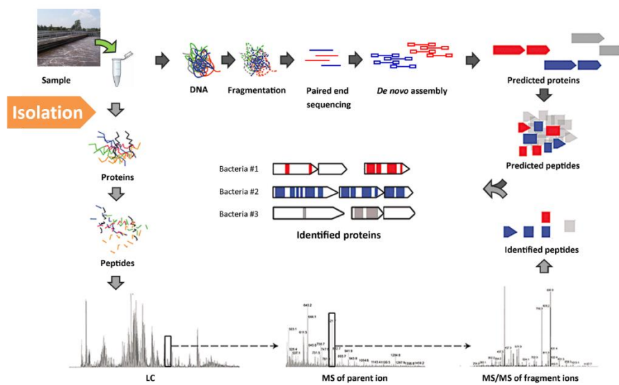
Figure 9 - Schematic overview of the metaproteomic approach combined with metagenomics. Modified from Denef et al. (2009).
