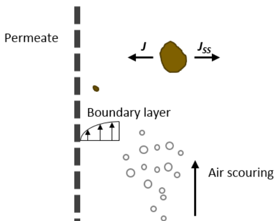
Figure B4 - Transport mechanisms in cake build-up.
