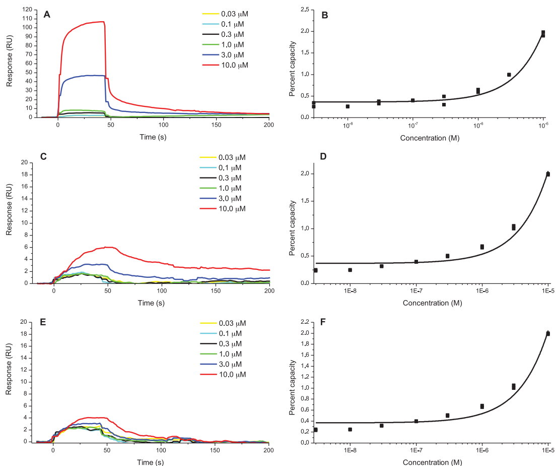
FIGURE 3. A, C, and E, sensorgrams showing the interaction of pyocyanin (A), PQS (C), and 3-oxo-C12-HSL (E) with FapC fibrils at concentrations ranging from 0.03 to 10 μM. B, D, and F, dose-response curves for the interaction between pyocyanin (B), PQS (D), and 3-oxo-C12-HSL (F) and FapC fibrils. Data are fit to a non-linear dose-response curve ( i.e. sigmoidal), with 100% site occupation determined from extrapolation. RU, response units.
