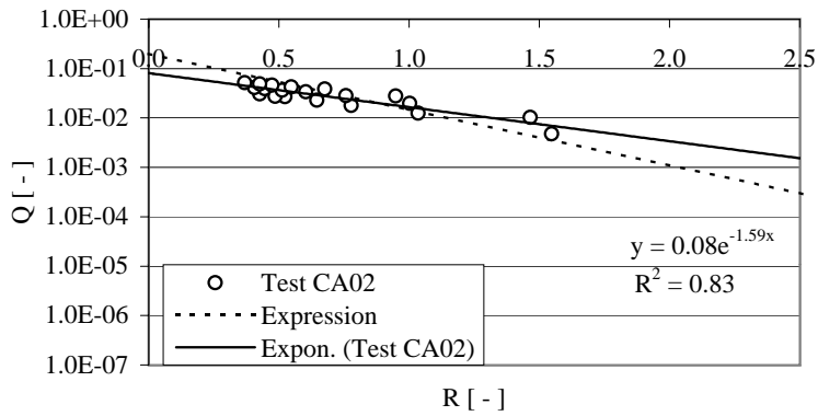
Figure B.24: Results of tests with test geometry CA02.
