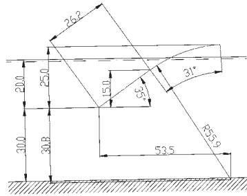
Figure B.27: The geometry of the slope in the CB01 tests. Measures are in cm.
