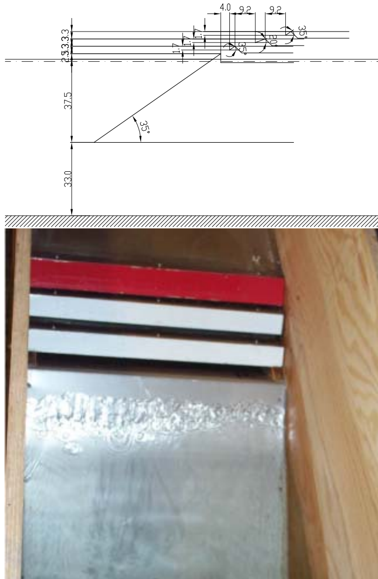
Figure C.12: Drawing (top) and photo (bottom) of model test setup C1, model scale. Measures are in cm.
