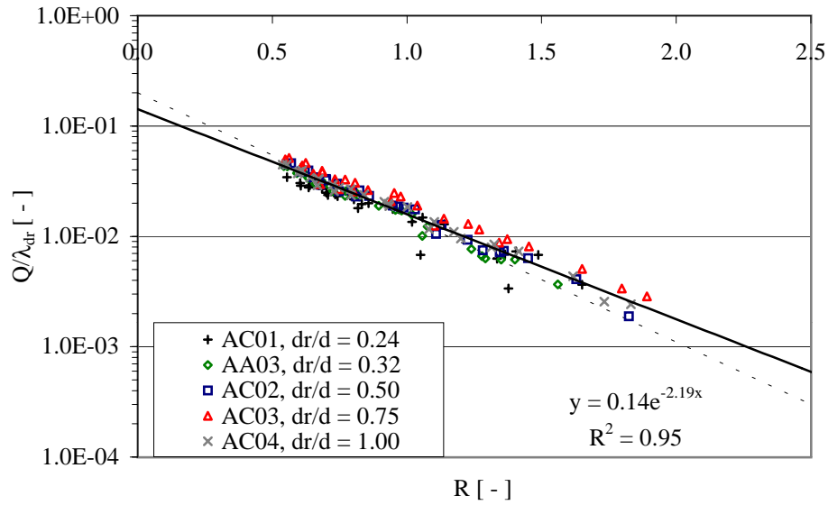
Figure 3.12: Results of tests with test geometries with varying d_r (test series AC). The dimensionless average overtopping discharge Q divided by the correction factor \lambda_{d_r} , is plotted as a function of the dimensionless crest freeboard R . The dotted line represents eq. 2.1 and the solid line is an exponential fit with all the data points shown.
