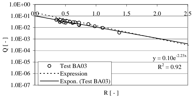
Figure B.20: Results of tests with test geometry BA03.
