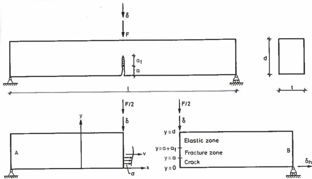
Fig. 2.4 The considered beam divided into two substructures, Brincker and Dahl (1989).
