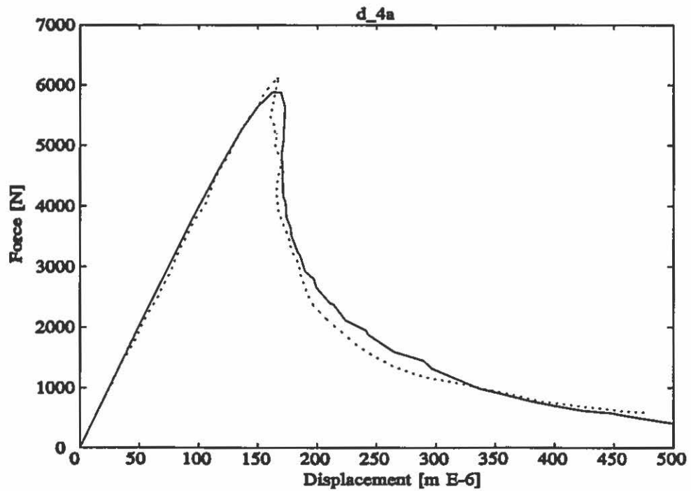
Figure A2.16: Fitted results for beam D-4.
