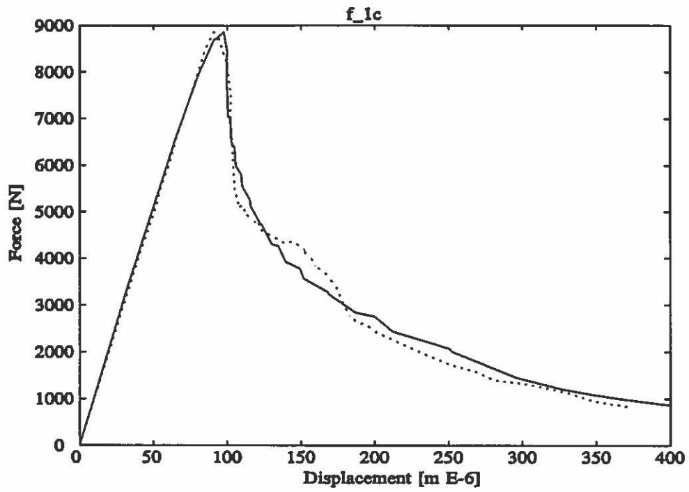
Figure A2.23: Fitted results for beam F-1.
