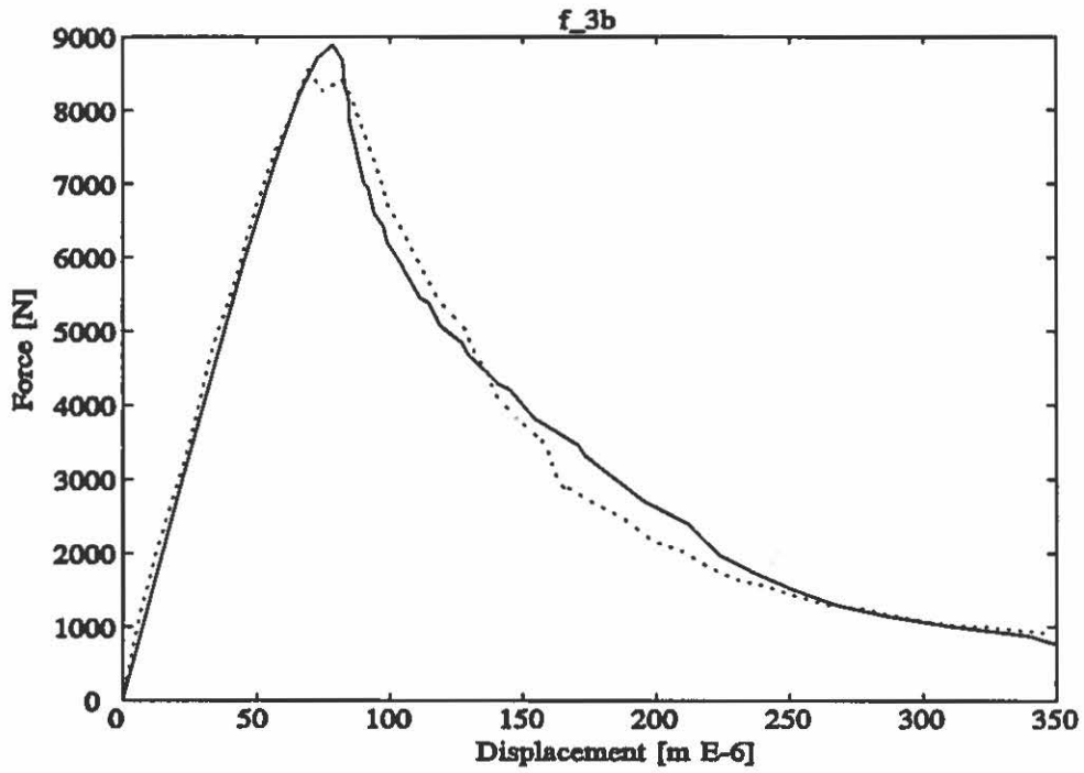
Figure A2.25: Fitted results for beam F-3b.
