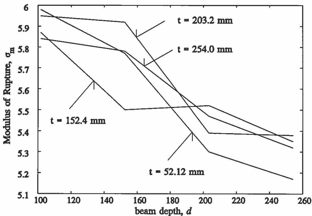
Fig. 2.18: Modulus of rupture for varying values of the beam depth, d , and thickness, t , and span equal to 762 mm, Willis and Reagal (1931).
