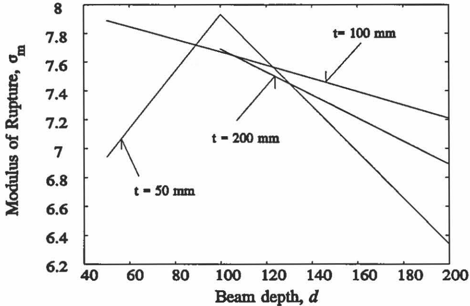
Fig. 5.11 Mean values of modulus of rupture as function of the beam depth for the three beam thickness.
