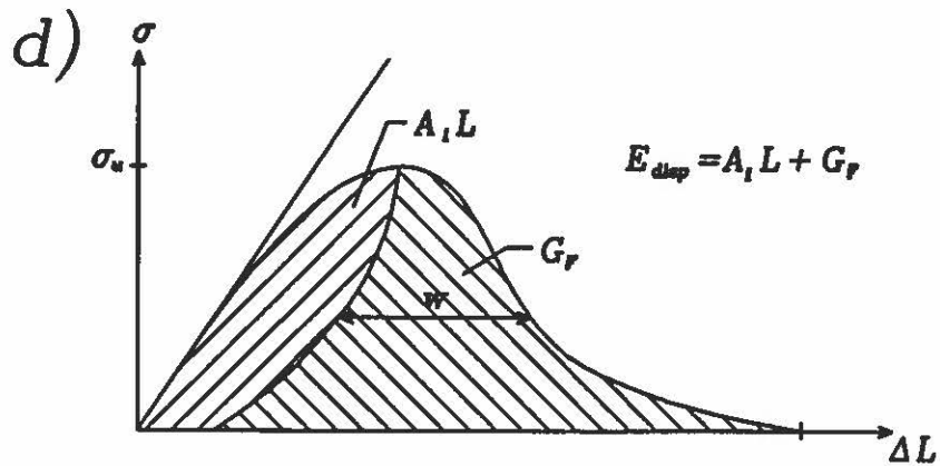
Fig. 2.11: The total elongation of a rod can be divided into three parts. a) linear elastic part b) non-linear in-elastic part and c) localized part. d) the total elongation.
