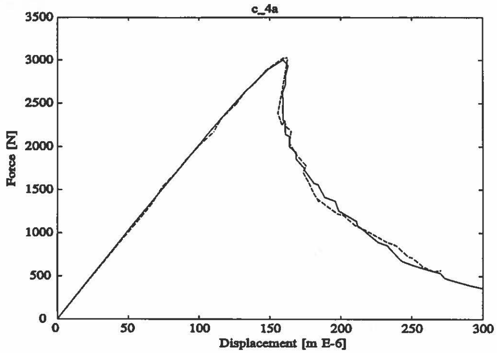
Figure A2.11: Fitted results for beam C-4.
