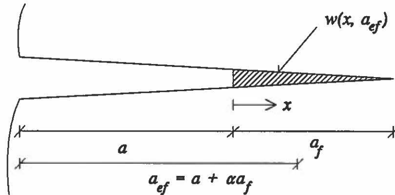
Fig. 2.17: Fictitious crack with an effective crack length.
