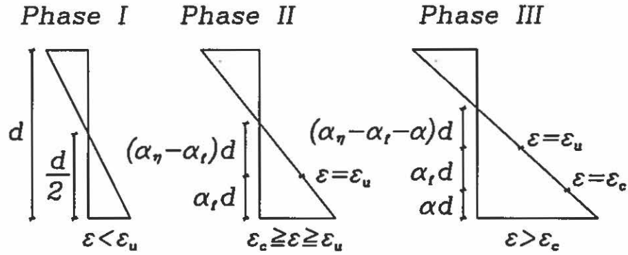
Fig. 4.16. Strain distribution in the three phases.
