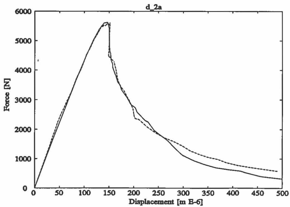
Figure A2.14: Fitted results for beam D-2.
