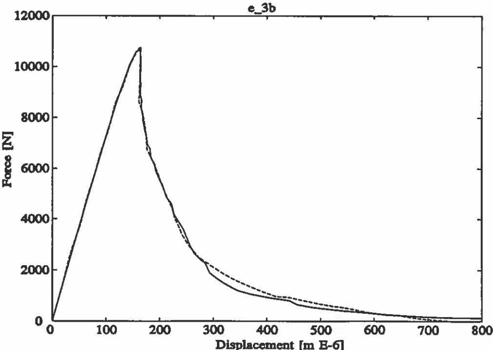
Figure A2.20: Fitted results for beam E-3.
