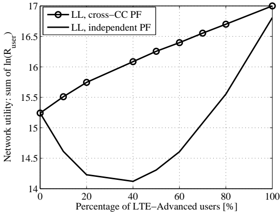
Fig. 4.7: Network utility with different ratios of the LTE-Advanced users. LL balancing is used, with 10 full buffer users per cell.
