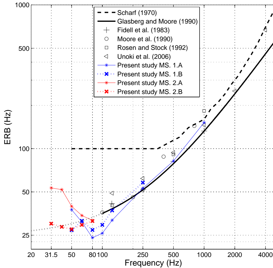
Figure 7: As figure 3 (see section 1.1), but mean ERB values from the present work have been included. Results described in Manuscript 1 (MS. 1) are shown in blue lines and symbols; 1.A: values obtained considering the combined filtering effects of the (assumed) middle-ear-transfer function and the derived filter shapes; 1.B: values obtained after including the middle-ear-transfer function as part of frequency selectivity below 50 Hz, but excluding it from frequency selectivity elsewhere. Results described in Manuscript 2 (MS. 2) are shown in red lines and symbols; 2.A: ERB values calculated for the mean psychophysical tuning curves; 2.B: ERBs of mean tuning curves; these were obtained after including the estimates of the middle-ear-transfer function as part of frequency selectivity only within the region of dominance of the helicotrema shunt.
