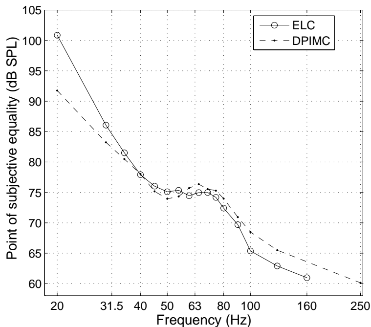
Figure 9: Example equal-loudness contour (ELC) and distortion-product-isomodulation curve (DPIMC) obtained for an individual (subject 6). The y-axis shows the measured levels corresponding to the ELC. The DPIMC has been vertically shifted to match the ELC. More results and details can be found in Manuscript (4).
