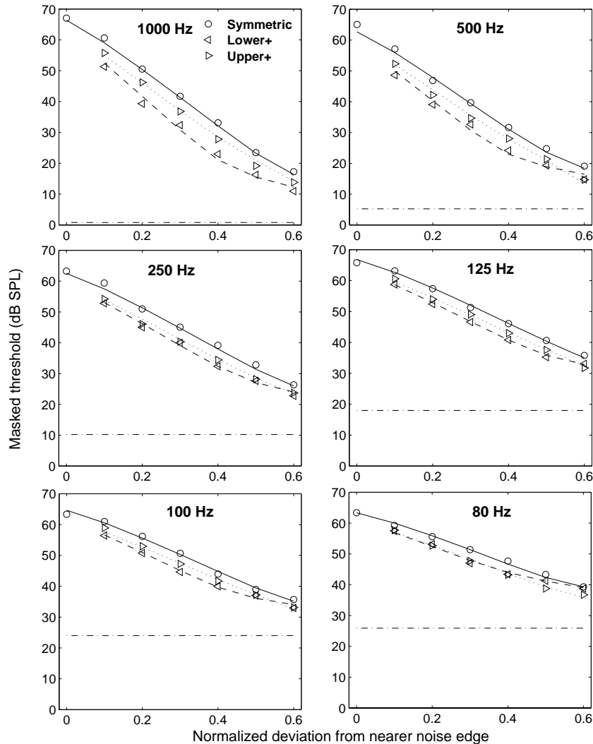
FIG. 3. Mean masked thresholds and fits from the model for f_s = 1000, 500, 250, 125, 100, and 80 Hz. Thresholds for symmetric-notch conditions are denoted by circles and corresponding fits by solid lines. Thresholds for 'lower+' conditions are denoted by left-pointing triangles and corresponding fits by dashed lines. Thresholds for 'upper+' conditions are denoted by right-pointing triangles and corresponding fits by dotted lines. Mean absolute thresholds are shown by horizontal dashed-dotted lines.
