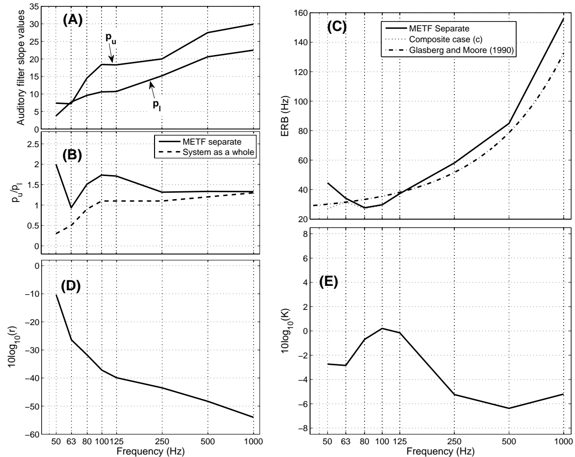
FIG. 5. (A): derived auditory filter slope parameters ( p values) for the METF-separate analysis; (B): asymmetry parameter, A , for the METF-separate and System-as-a-whole analyses (solid and dashed lines, respectively); (C): ERB values obtained for the METF-separate analysis (solid line), the analysis treating the METF as part of frequency selectivity for frequencies below 50 Hz ('composite' case, dotted line). The ERB values predicted by Eq. 1 are plotted as the dashed-dotted line; (D): values of the dynamic range parameter, r (dB) for the METF-separate analysis; (E): values of the detection efficiency parameter, K (dB), for the METF-separate analysis. In all cases (A to E) for f_s = 63 and 50 Hz, values are based on the data obtained with LF emphasis.
