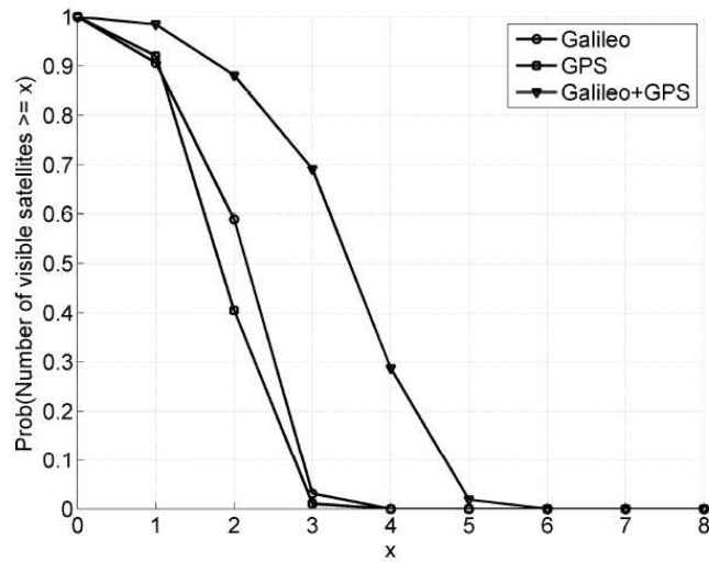
Figure 2.4: CDF of number of visible satellites ( x ) in urban canyon from [Mensing et al., 2008].
