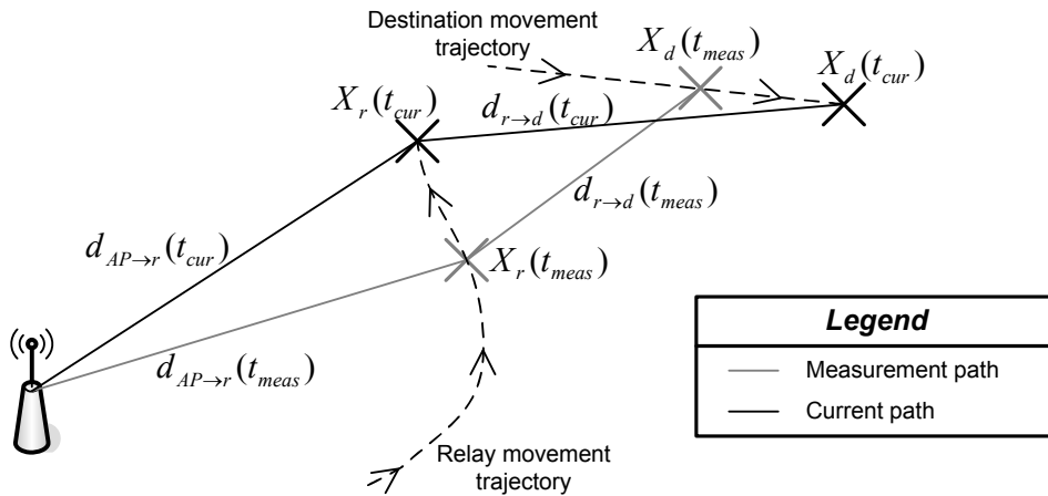
Figure 5.3: Node movements and aged measurements introduce errors in the node position and link distance knowledge. X denotes a node position, d is a link distance, t_{meas} is the time of the latest measurement, and t_{cur} is the current time.
