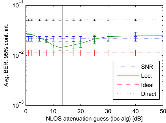
Figure 5.23: BER impact for different guesses of the unknown NLOS attenuation with a true value of 13.3dB . Wall is halfway between AP and bottom.
