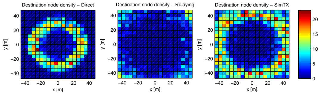
Figure 6.9: Density of destination node positions for each algorithm, based on 2500 runs.
