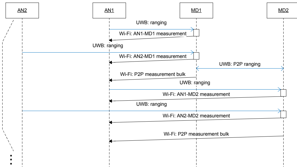
Figure 4.8: Sequence chart for an example scenario with 2 ANs and 2 MSs. In this example AN1 is closer to both MSs than AN2, and the MSs therefore send their obtained measurements through the AP in AN1. The UWB ranging measurement procedure is depicted with blue arrows.
