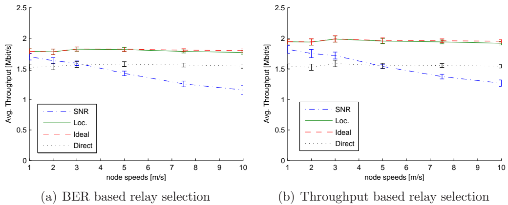
Figure 5.14: Throughput impact of varying node speed.
