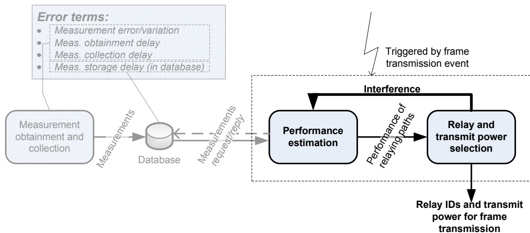
Figure 6.2: Extended version of the general relaying system in Figure 5.2. The greyed-out parts are not considered in details in this chapter, whereas the bold text shows the additions.
