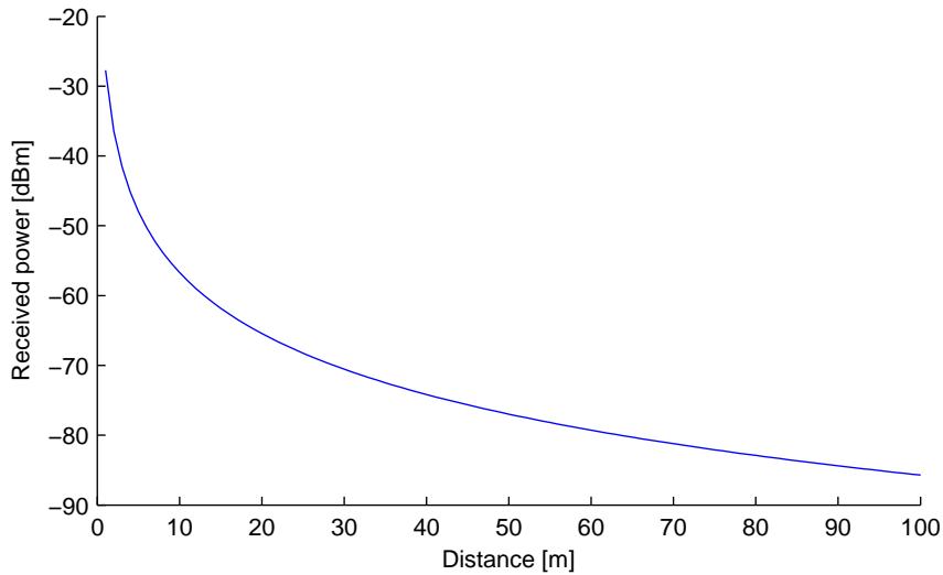
Figure 2.2: Example of received power for P_{tx} = 20\text{ dBm} , PL(d_0) = 0 , and n = 2.9 .
