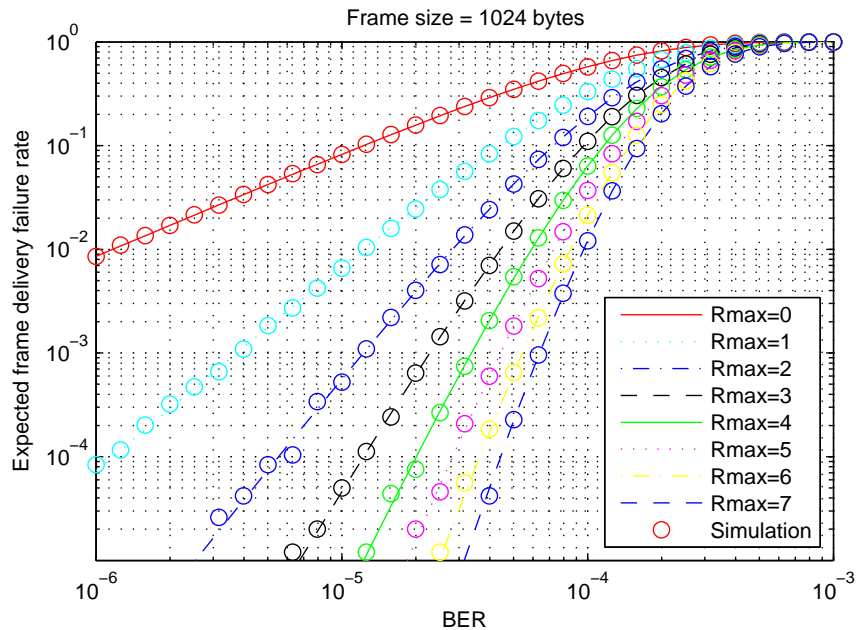
Figure 3.2: Expected FER ( 1 - P_{\text{succ}} ) for 6 Mbit/s and B_{\text{MSDU}} = 1024 bytes.
