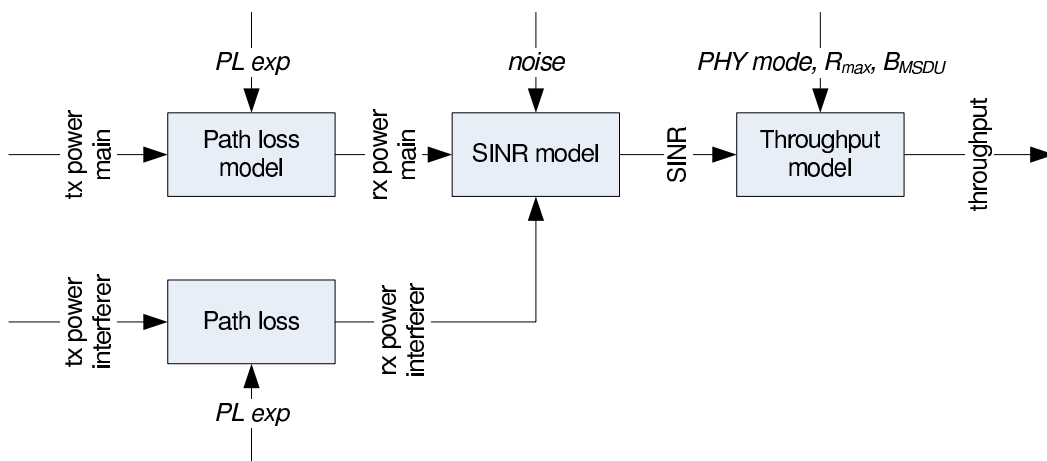
Figure 3.1: Structure of throughput model. Model parameters are italicized.
