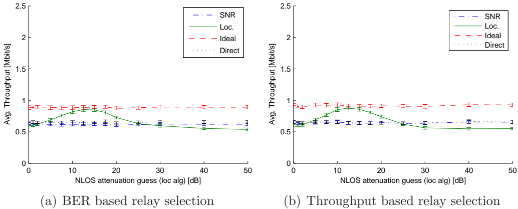
Figure 5.24: Throughput impact for different guesses of the unknown NLOS attenuation with a true value of 13.3dB . Wall is halfway between AP and bottom. Tx power is 300 mW.
