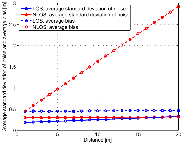
Figure 4.2: Average ranging error model parameters vs. distance
