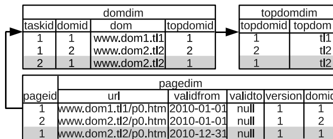
Figure 4.7: Before post-fixing
