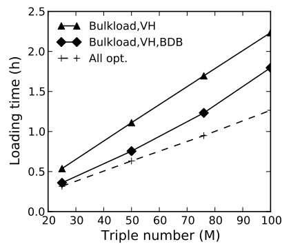
Figure 2.8: Bulkload optimizations
