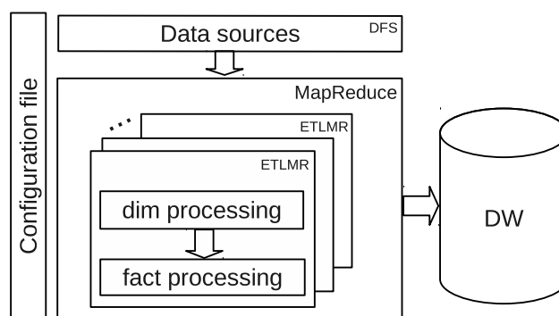
Figure B.1: Parallel ETL using ETLMR
