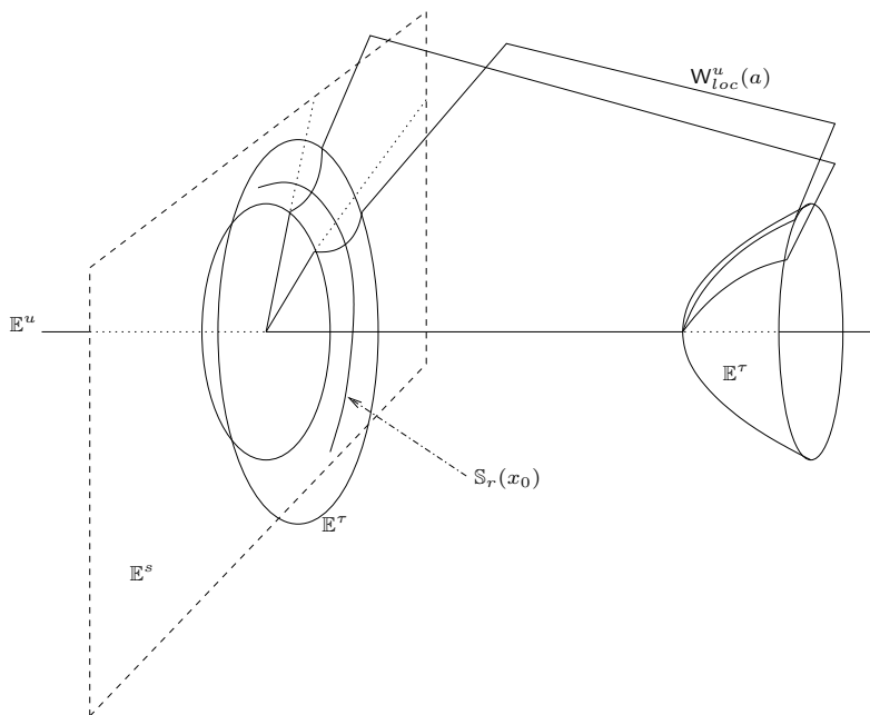
Figure 4.5: A graphic interpretation of the construction in the proof of lemma 4.12, with k = 2 . Note that \mathbb{S}_r(x_0) is only partially illustrated.
