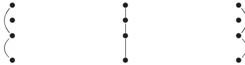
Figure 4.9: The progress of \rho on J \subset S , where \bullet denote the critical points q , b , a and p listed from below. Hence \rho(s)(\kappa) is in the zero section of the disk bundle for all s \in J .
