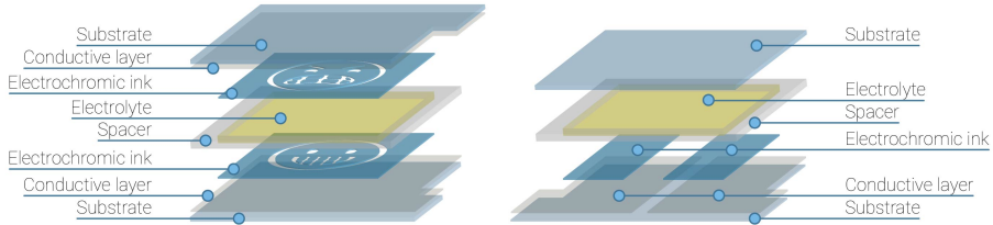
Fig. A.3: Composition of vertical stacked electrochromic technology.
