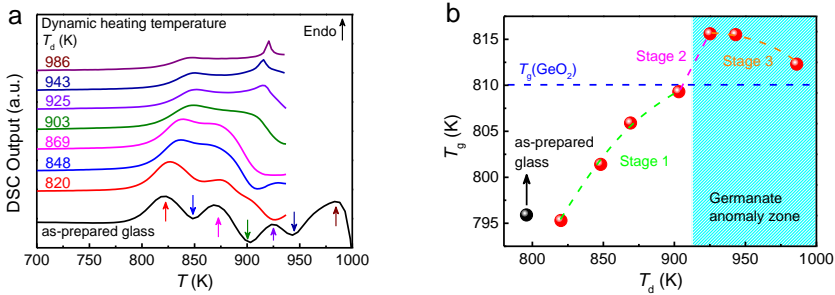
Figure 3-11 (a) DSC first upscan curves of the glasses dynamically heated to different T_d . Arrows show the temperature positions of T_d . (b) The evolution of T_g with T_d , exhibiting three stages illustrated by the dashed curves. T_g(\text{GeO}_2) is the glass transition temperature of the \text{GeO}_2 glass. The blue region displays the possible germanate anomaly zone.
