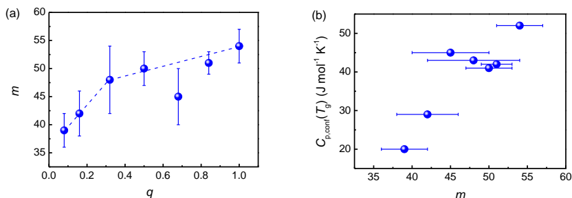
Figure 4-2 (a) Composition dependence of liquid fragility m . q represents the mole ratio of [B_2O_3]/[B_2O_3]+[SiO_2] . (b) Relation between C_{p,conf}(T_g) and liquid fragility index m of studied borate-silicate glasses.
