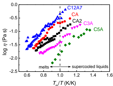
Figure 4-7 T_m scaled viscosity of studied CaO-Al 2 O 3 liquids in the temperature region of 1500-2800 K.
