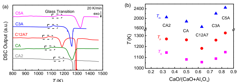
Figure 3-14 (a) DSC first upscan of studied CaO-Al 2 O 3 glasses at 20K/min. (b) Composition dependence of glass transition temperature ( T_g ), crystallization peak temperature ( T_p ), and melting temperature ( T_m ). T_m is obtained from the binary phase diagram of CaO-Al 2 O 3 .
