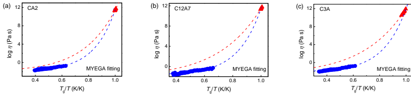
Figure 4-9 Viscosity of three studied CaO-Al 2 O 3 liquids (a) CA2, (b) C12A7, and (c) C3A in the temperature region near T_g and around T_m . Dashed lines refer to MYEGA fittings.
