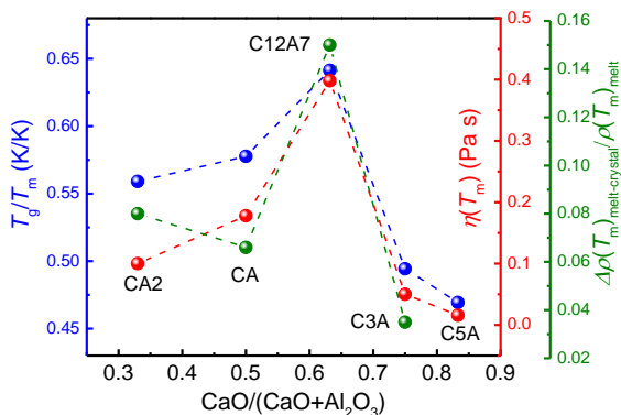
Figure 5-5 GFA metrics T_g/T_m , \eta(T_m) , and \Delta\rho(T_m)_{melt-crystal}/\rho(T_m)_{melt} . The density data of crystals and melts are obtained from MD simulation.
