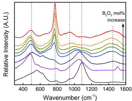
Figure 2-2 Raman spectra for \text{Na}_2\text{O-CaO-B}_2\text{O}_3\text{-SiO}_2 glasses.
