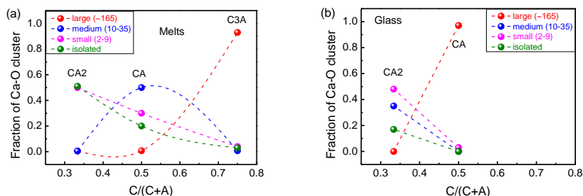
Figure 2-16 Distribution of clusters containing CaO_x polyhedra with various sizes for CaO-Al_2O_3 (a) melts and (b) glasses. Out of 172 units: Large ~165 units (red), Medium 10-35 units (blue), Small units 2-9 units (pink), Isolated units (olive).
