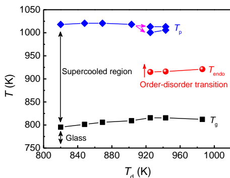
Figure 5-3 Characteristic temperatures ( T ) as a function of the dynamic heating temperature ( T_d ) for 60\text{GeO}_2\text{-}25\text{BaF}_2\text{-}15\text{AlF}_3 glass system. T_g , T_{endo} , and T_p refer to the glass transition temperature, the peak temperature of the endotherm characterizing the order-disorder transition, and the crystallization peak temperature, respectively. The pink arrows show the splitting of the crystallization peak into two sub-peaks.
