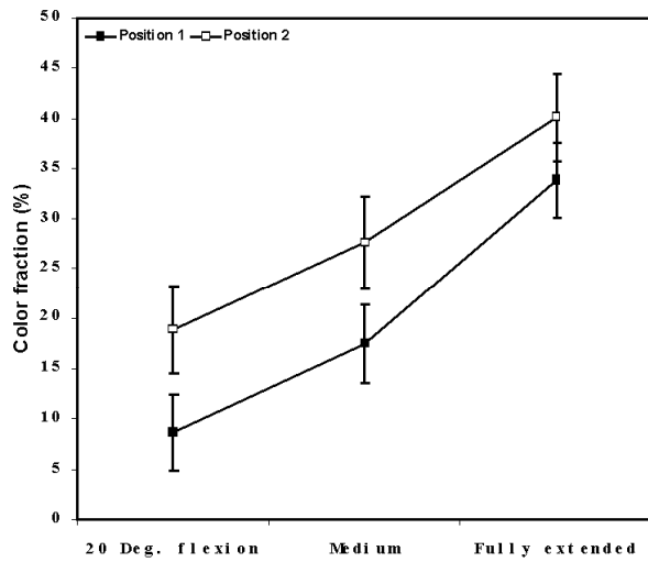
Figure 9. Effect of knee position on color fraction and resistive index. The graphs with filled boxes are with full extension as initial position. Values are presented as (least-squares) means \pm standard error of the mean (SE). Left: Color fraction (CF) as function of knee position. The decrease in CF with increasing flexion was highly significant (P for trend <0.0001 ). Right: Resistive index (RI) as function of knee position. The increase in RI with increasing flexion was highly significant (P for trend <0.0001 ).
