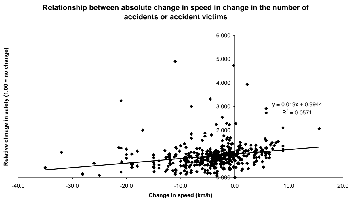
Figure 20: The linear model of the relationship between changes in speed and changes in road safety
