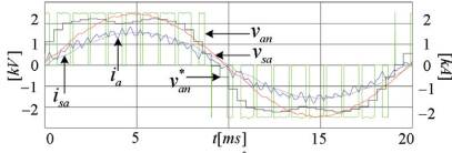
Fig. 7. The phase- \alpha reference voltage v_{am}^* , converter voltage v_m , converter current i_m , grid voltage v_{sa} , and grid current i_{sa} waveforms for 3L-HB/C-VSC at P=6\text{MW} and \text{PF}=1
