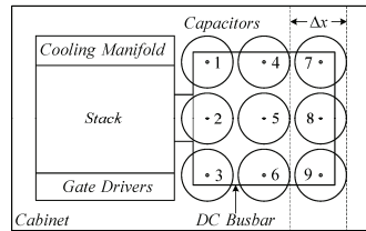
Fig. 15. Top view of the 3L-HB-VSCs' cabinet
