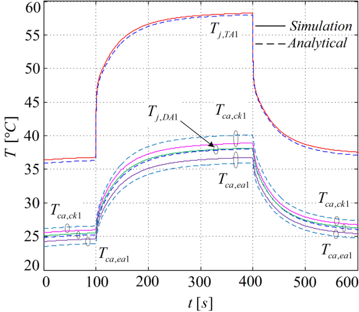
Fig. 3.26. Comparison of the converter-leg thermal model simulation and analytical solution results for the transitions between 1.5MW and 3MW where PF=1 , T_{cw}=T_{amb}=15^{\circ}C , and v=5l/min
