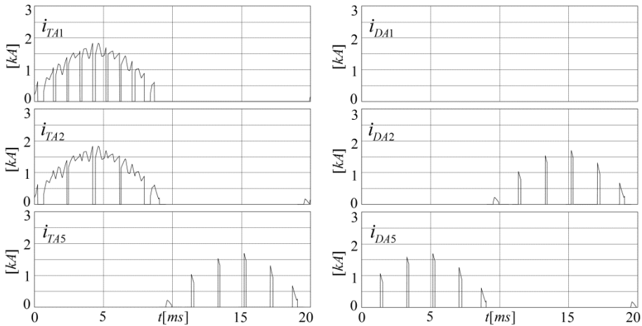
Fig. 2.25. Phase- a switch current waveforms i_{TA1} , i_{DA1} , i_{TA2} , i_{DA2} , i_{TA5} , i_{DA5} for 3L-ANPC-VSC at P_{DC}=6\text{MW} and \text{PF}=1
