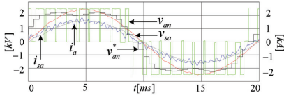
Fig. 8. The phase- \alpha reference voltage v_{am}^* , converter voltage v_m , converter current i_m , grid voltage v_{sa} , and grid current i_{sa} waveforms for 3L-FB/S-VSC at P=6\text{MW} and \text{PF}=1
