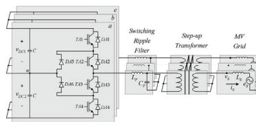
Fig. 1. Three-phase 3L-NPC-VSC connected to a MV grid
