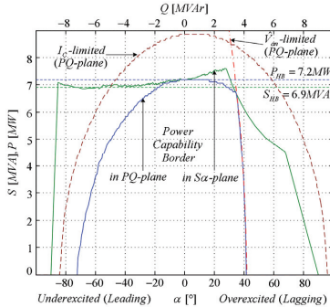
Fig. 13. Power capability of the 3L-HB-VSCs in PQ- and Sα-plane
