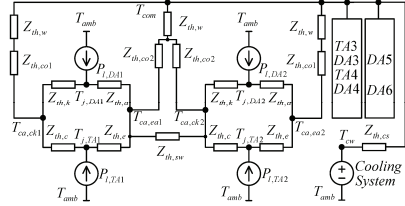
Fig. 10. Dynamical thermal model of the converter phase-a leg
