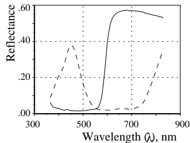
Figure 5.9: Reflectance of the red enameled cup (solid curve) and the blue vacuum jug (dashed curve), obtained by a spectrometer designed and manufactured by VTT, Oulu, Finland.
