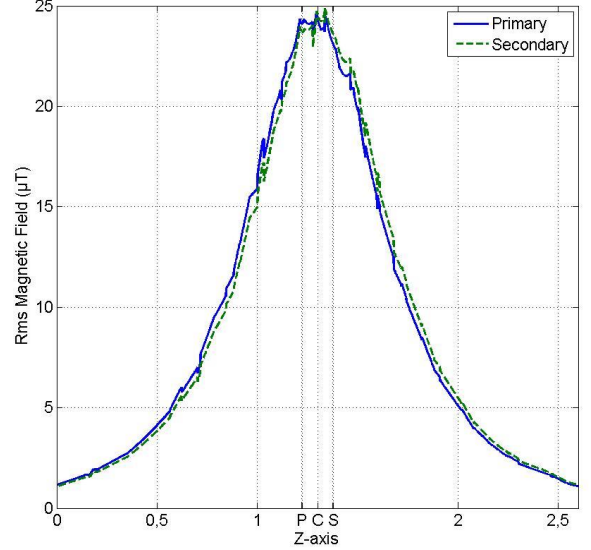
Fig. 5. Rms magnetic field ( \mu\text{T} ) versus Z-axis – No-load [5]
