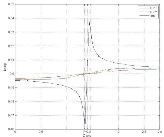
Fig. 10 Ratio K_s/K_p versus Z-axis at V=10\text{cm} , T=12:6 .
