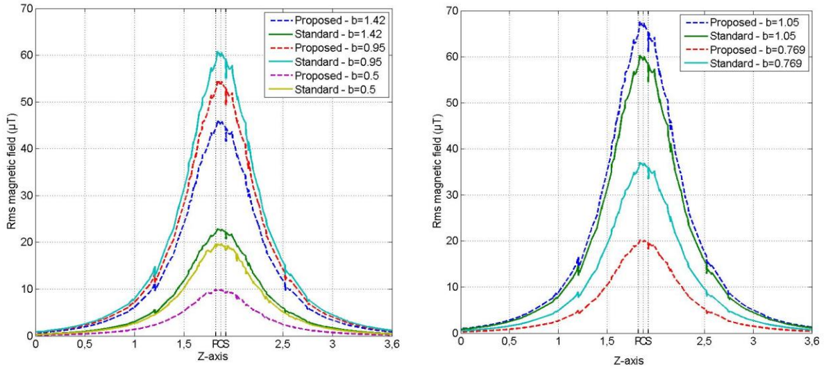
Fig. 8: Rms magnetic field ( \mu\text{T} ) versus Z-axis – Aligned case
