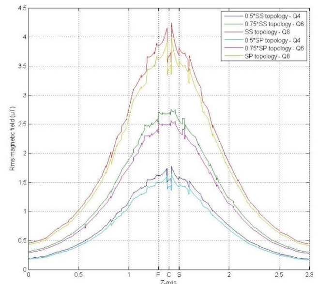
Fig. 13 On-load - Rms magnetic field ( \mu\text{T} ) versus Z-axis at V=20cm, T=12:12.
