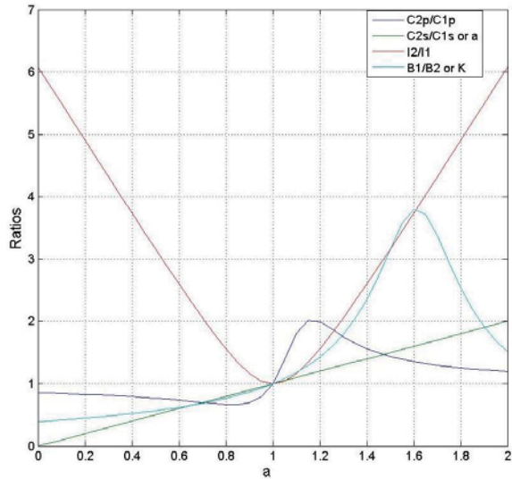
(a) K_s/K_p=1 , M/L_s=0.38 , Q=6
