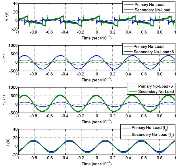
(b) Electrical quantities
