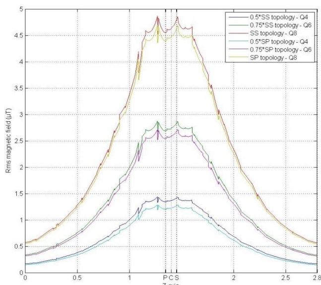
Fig. 11 On-load - Rms magnetic field ( \mu\text{T} ) versus Z-axis at V=10cm, T=12:12.
