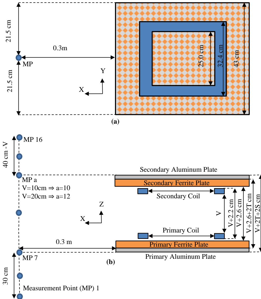
Figure 1 – Inductor setup
