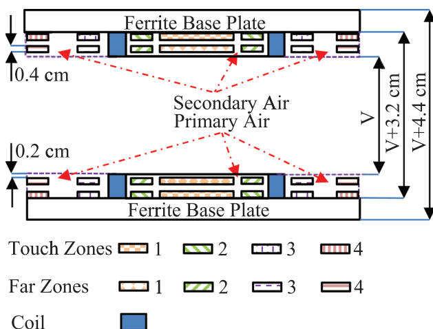
FIG. 2. Sample geometry top view.
