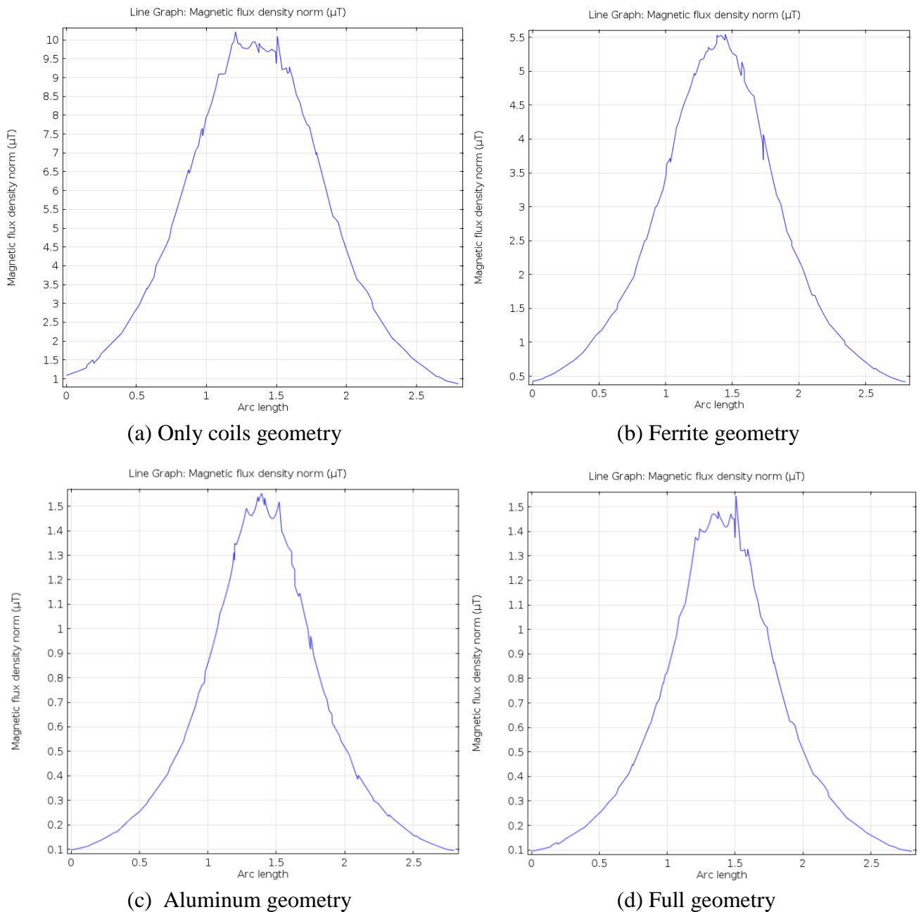
Figure 13. Magnetic emissions ( \mu\text{T} ) versus Z-axis
