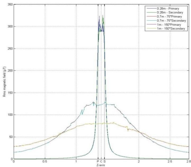
Fig. 7 No-load - Rms magnetic field ( \mu\text{T} ) versus Z-axis at V=10\text{cm} , T=12:12 .
