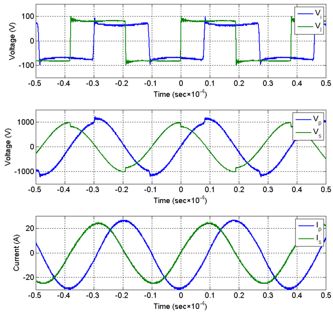
(c) Electrical quantities at Q_{I2}
