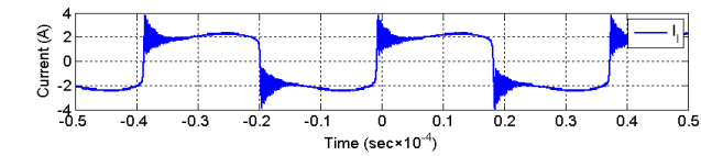
(c) Electrical quantities at Q_{12}
