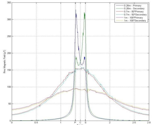
Fig. 9 No-load - Rms magnetic field ( \mu\text{T} ) versus Z-axis at V=20\text{cm} , T=12:12 .
