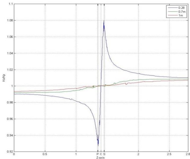
Fig. 6 Ratio K_s/K_p versus Z-axis at V=10\text{cm} , T=12:12 .
