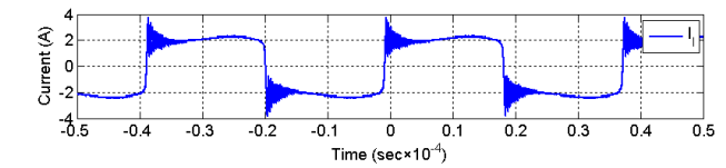
(b) Electrical quantities at Q_{11}
