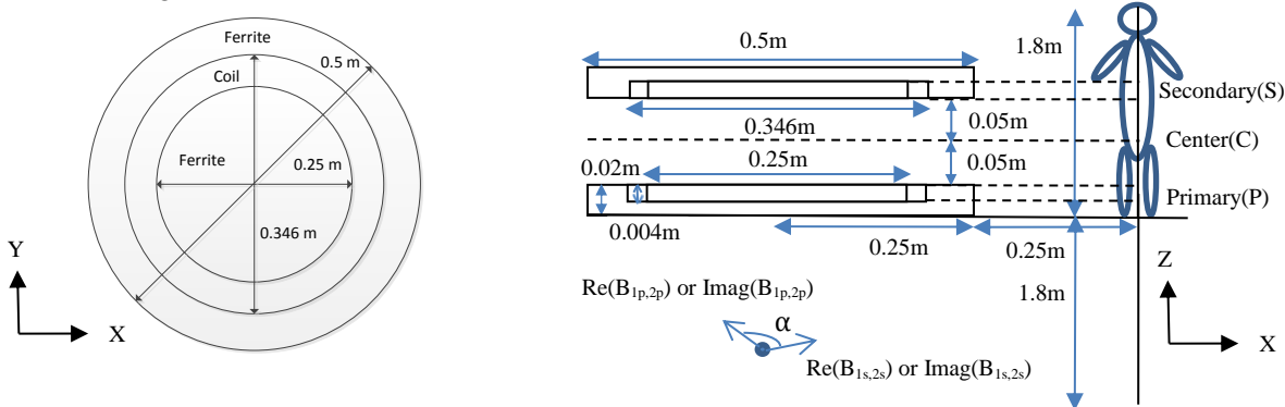
Fig. 2: Top and side views sample geometry [7]
