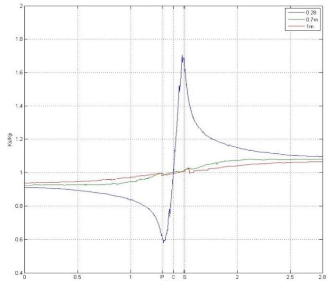
Fig. 8 Ratio K_s/K_p versus Z-axis at V=20\text{cm} , T=12:12 .
