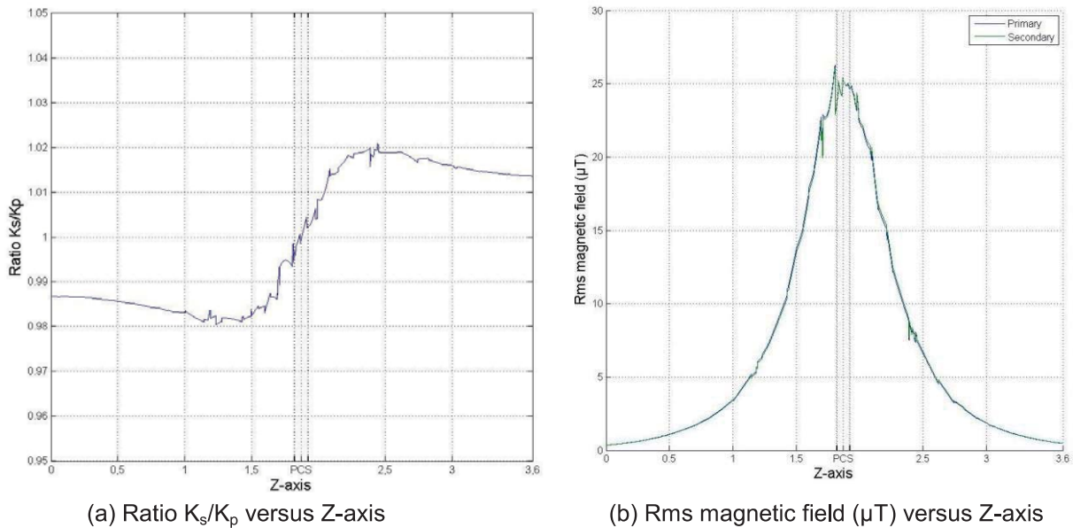
Fig. 5: No-load curves [7]
