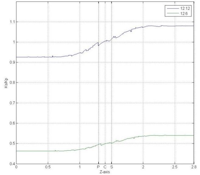
Fig. 8 Ratio K_s/K_p versus Z-axis at V=20\text{cm} .
