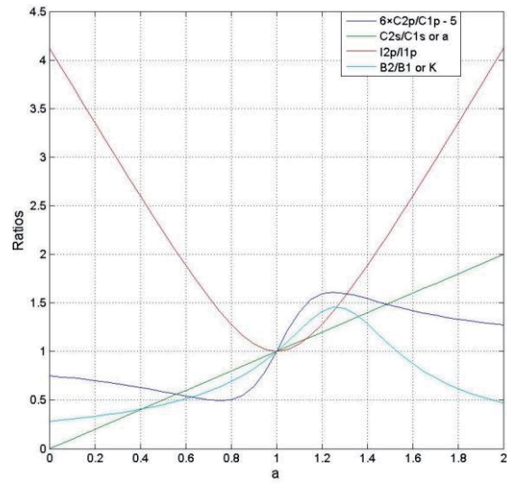
(b) K_s/K_p=1 , M/L_s=0.21 , Q=4
