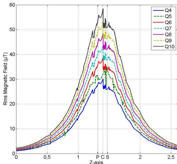
Fig. 8. Rms magnetic field ( \mu\text{T} ) versus Z-axis – On-load
