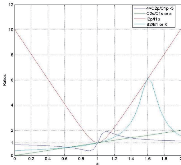
(c) K_s/K_p=2 , M/L_s=0.19 , Q=10
