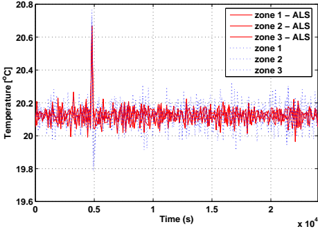
Figure 3.12: Comparison of Closed loop Performances for Set-point Tracking with ALS and Nominal Estimator
