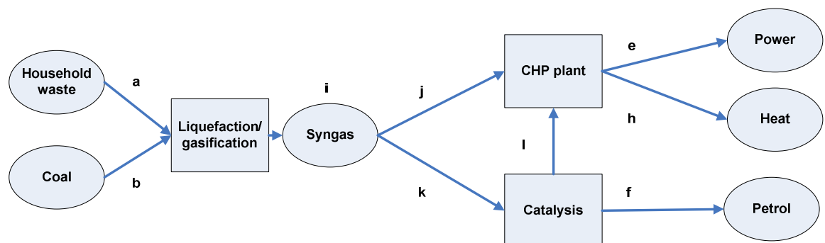
Figure 2 Gasification with use for CHP and transport
