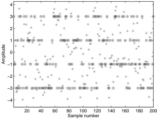
Figure 10: The recovered symbol sequences. Dots: the transmitted symbols, circles: the recovered symbols by the HMARM, stars: the recovered symbols by the LS method.
