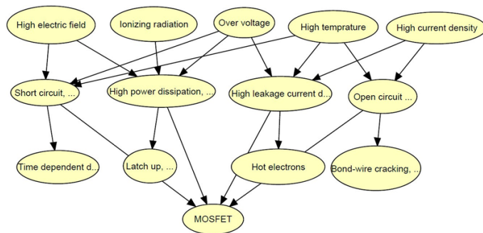
Figure 2-2: Bayesian Network for the MOSFET (Rastayesh, Bahrebar, et al., 2020).
