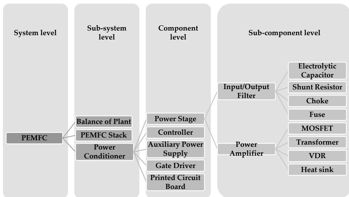
Figure 1. Simplified schematic of the proton exchange membrane fuel cell (PEMFC) categorized in different levels.
