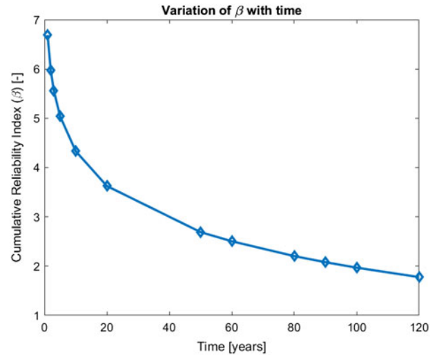
Figure 5. Variation in Cumulative reliability index along service duration of structure (FDF \sim 2 and T_L=120 years).
