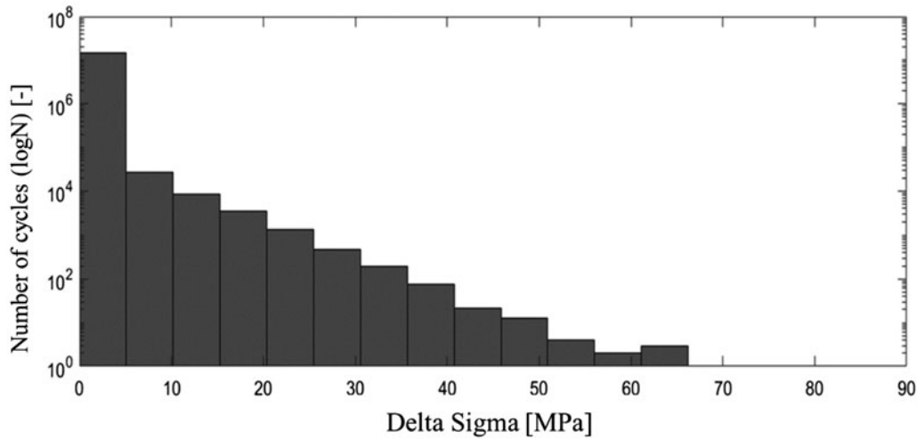
Figure 4. Stress histogram for transverse reinforcement.
