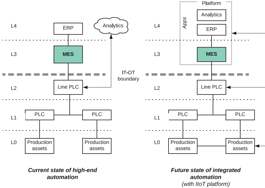
Fig. 2: ISA 95 hierarchy of systems with IIoT interconnectivity [16]
