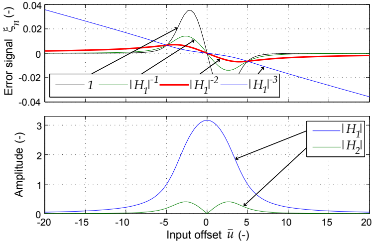
Figure 7.4: Error signal normalized with 1 , |H_1|^{-1} , |H_1|^{-2} , and |H_1|^{-3} at different input offsets, together with the corresponding amplitude of the first and second harmonic.
