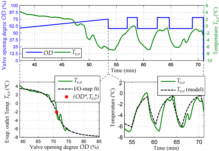
Figure 2.19: Ramp and relay feedback test on a MT open shelf type display case in the CO 2 supermarket refrigeration system.
