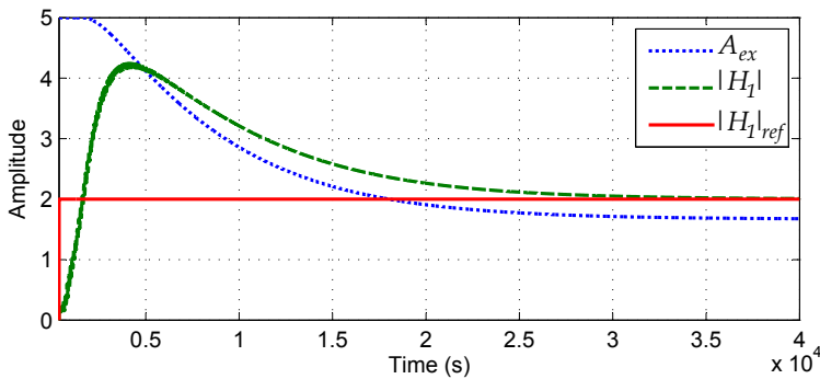
Figure 5.10: Adaptation of the excitation signal amplitude A_{ex} during the simulation shown in Fig. 5.9. The amplitude of the first harmonic |H_1| is used as feedback signal.
