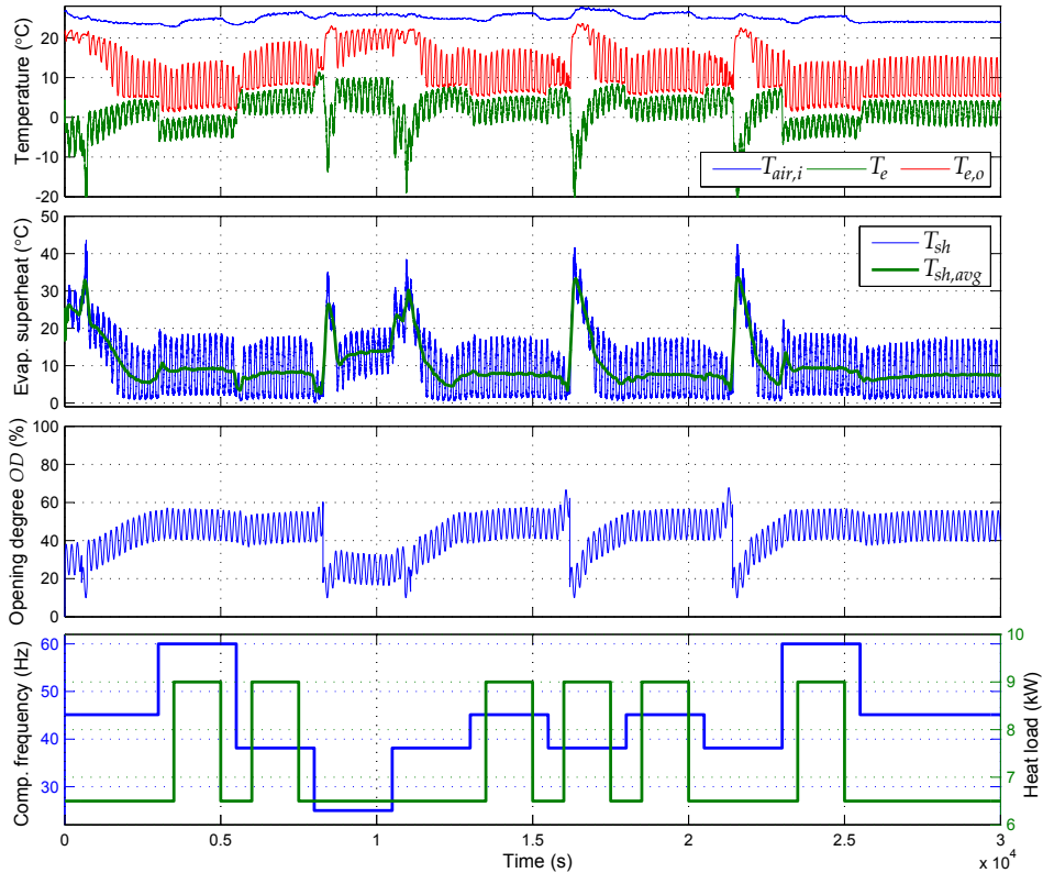
Figure 6.11: Test of the harmonic controller on the air conditioning system. The load in the bottom plot is approximately the heat applied to the air conditioned room using an electric heater. The same time scale is used for all four plots.
