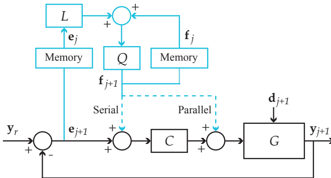
Figure 1.11: ILC (light blue) applied to a closed-loop system (black). Both serial and parallel ILC structure are shown.
