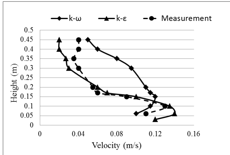
Figure 3.10 Prediction of velocity profile at a distance of 1 m in front of the inlet by k-\varepsilon and k-\omega compared with the measurement results (Paper VI)
