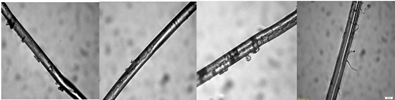
Figure 4.2 Photos from the filters with varying exposures a) <3.0E+4 b) 1.2E+5 c) 1.5E+6 d) 3.0E+6
