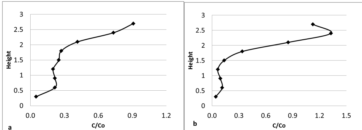
Figure 3.15 Predicted average particle concentration profile by k-\varepsilon + Radiation when the heater is at height 0.5 m and the particle source at heights a) 0.2 m b) 1.5 m
