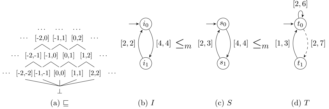
Figure 4.: Weighted modal automata over K_{weighted}
