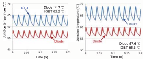
Fig. 14. Junction temperature in the grid-side converter (Wind speed: 12 m/s).
