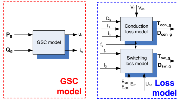
Fig. 2.6. Block diagram to calculate the power loss for the grid-side converter.
