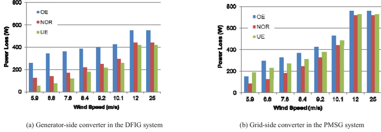
Fig. 13. Power loss profile of different system considering grid codes. Note: OE, NOR and UE indicate over-excited, normal and under-excited reactive power.
