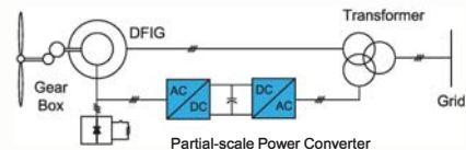
(a) Wind turbine system with partial-scale power converter
