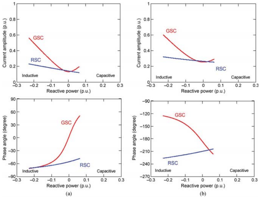
Fig. 6. Current characteristic of the back-to-back power converter at two different wind speeds. (a) Subsynchronous mode (wind speed: 5.9 m/s). (b) Supersynchronous mode (wind speed: 10.1 m/s).
