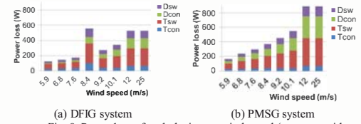
Fig. 9. Power loss of each device vs. wind speed (generator-side converter).
