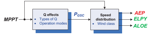
Fig. 13. Framework to predict the cost of energy loss in respect to the reactive power requirement from grid codes.
