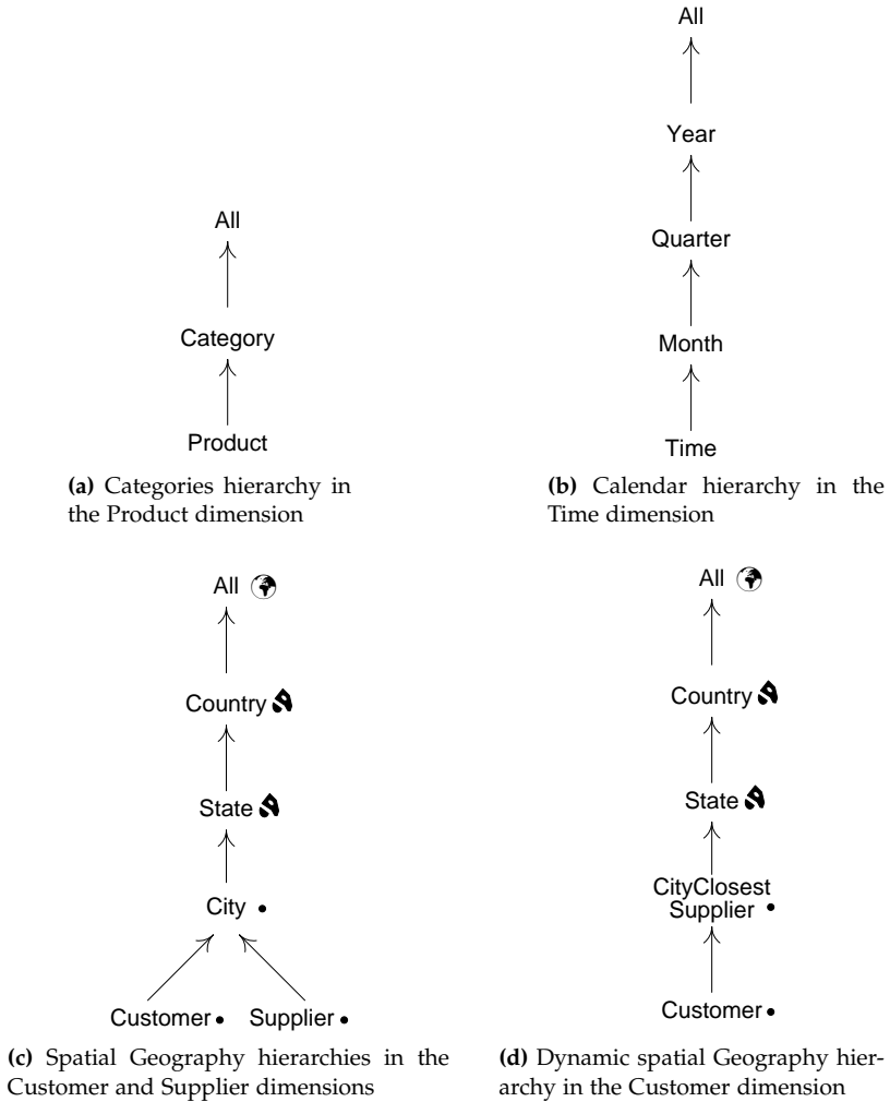
Fig. C.4: Dimension hierarchies
