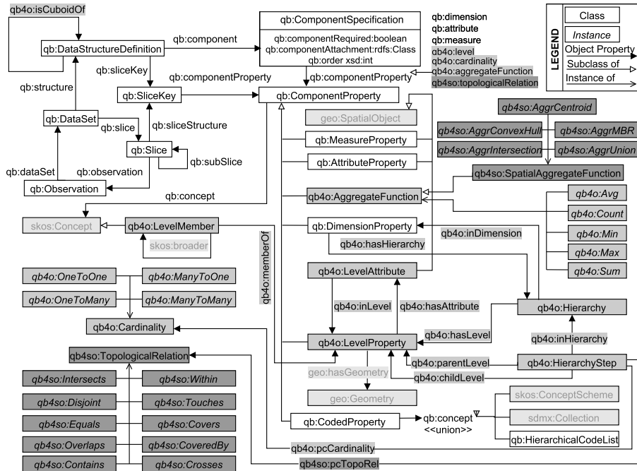
Fig. 9: The QB4SOLAP vocabulary (V1.3) (adapted from [15])
