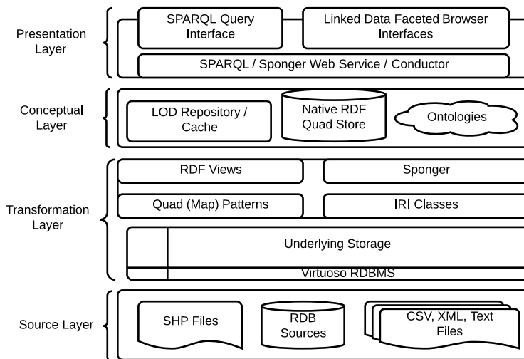
Fig. 6: Multi-layered system architecture (adapted from [4])
